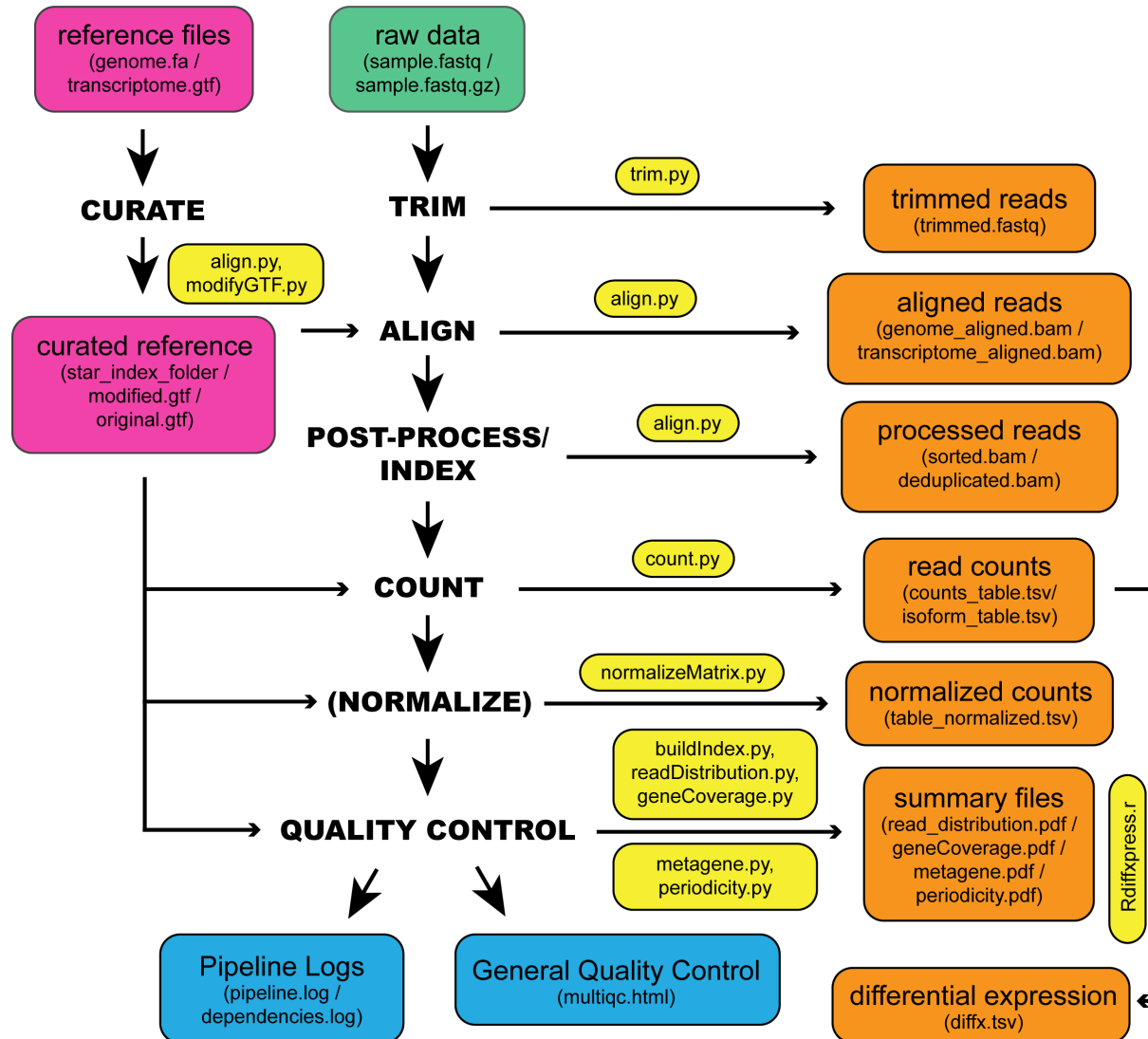
Figure 1: Workflow schematic of the inputs, outputs, and organization of XPRESSpipe. Representation of the general steps performed by XPRESSpipe with data and log outputs. Steps in parentheses are optional to the user. Input and output file types are in parentheses for each input or output block. The main script(s) used for a given step are in yellow blocks. The green block indicates input sequence file(s). Pink blocks indicate reference input files and curated reference. Orange blocks indicate output files. Blue blocks indicate general quality control and log file outputs. Differential expression analysis is run independently from the pipeline as the user will need to ensure count table and metadata table formatting are correct before use.
