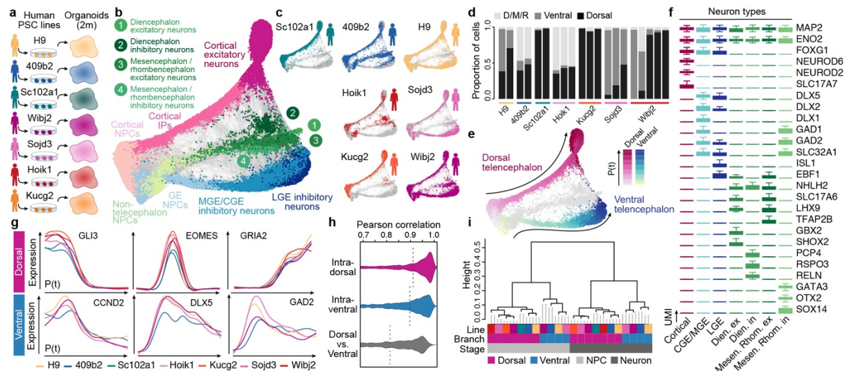
Figure 2: Assessing the reproducibility of gene expression patterns in the human organoid forebrain from iPSC lines from different individuals.
