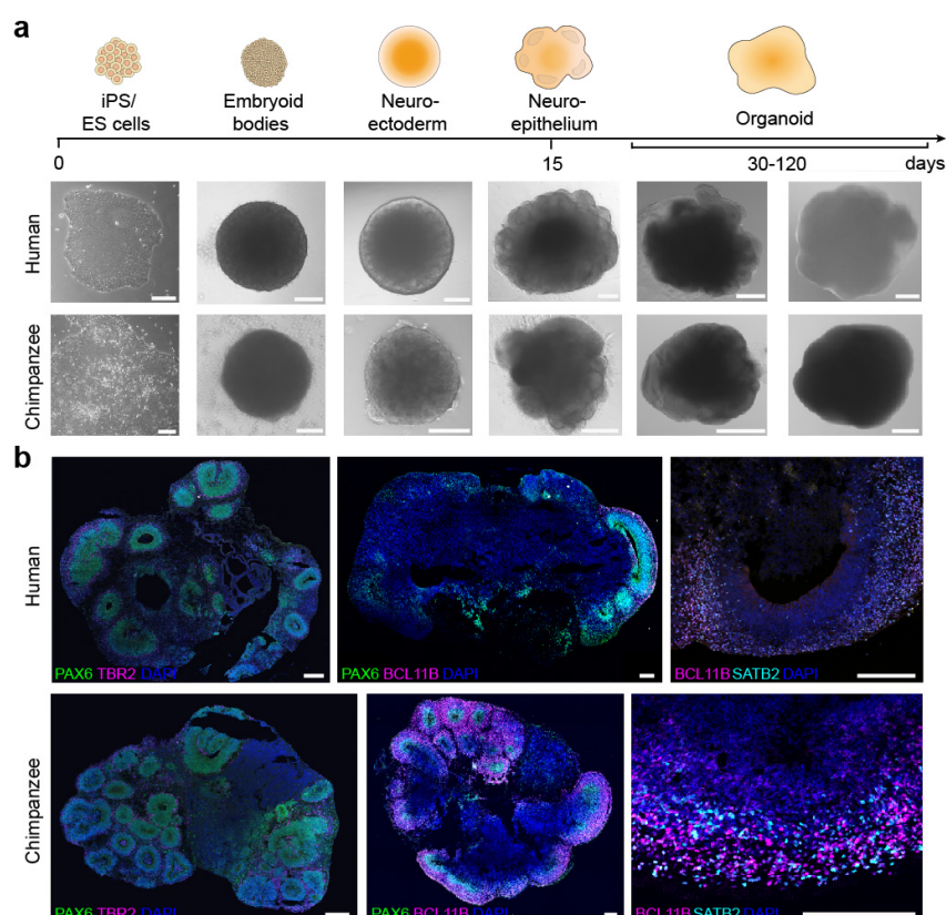
Extended Data Figure 1. Differentiation and immunohistochemical characterization of human and chimpanzee cerebral organoids. (a) Phase contrast (iPSC stage – neuroepithelium, scale bar 200 μm; H9 for human, SandraA for chimpanzee) and bright field images (organoid stages, scale bar 1 mm; H9 and Wibj2 for human, JoC and SandraA for chimpanzee) of different stages of organoid development for human and chimpanzee organoid differentiation. (b) Immunohistochemical stainings of human (Sc102a1 and 409b2) and chimpanzee (all SandraA) organoids reveal proper formation of cortical-like regions (scale bar 200 μm).
