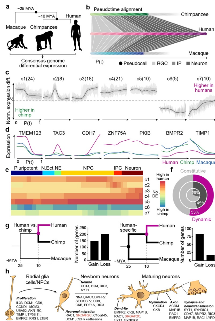
Figure 4: Identification of human-specific changes in corticogenic gene expression. (a) scRNA-seq was performed on 2-4 month-old organoids from human, chimpanzee and macaque lines. Reads were aligned to a consensus genome, to analyze human-specific gene expression. (b) A schematic of time warping alignment of pseudotimes of the cortical progenitor to deeper layer neuron trajectories in human, chimpanzee and macaque in order to perform differential gene expression analysis. (c) Differential expression analysis of the aligned data reveals 7 clusters of genes with distinct human-specific pseudotemporal expression patterns. Average differential expressions of cluster genes are plotted over pseudotime for organoid dorsal forebrain pseudocells with 50% and 95% confidence intervals shown in dark and light grey, respectively. The number of genes per cluster are shown in parenthesis. (d) Pseudotemporal expression pattern of exemplary genes with human-specific expression changes for each of the 7 clusters, comparing human (pink), chimpanzee (green) and macaque (blue) expression. (e) Average human-chimpanzee differential expression patterns along the trajectory from pluripotent cells to cortical neurons shown for the 7 clusters of genes with human-specific pseudotemporal expression changes in organoid cells. (f) Proportions of genes with pseudotime-dependent (dynamic, dark) or constitutive expression patterns (grey), in all (inner), expression-controlled (outer) organoid cells.
