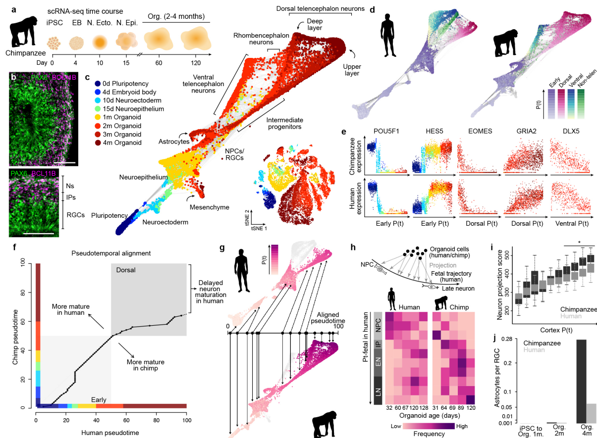
Figure 3: Chimpanzee cerebral organoid reconstructions reveal heterochrony in early cortex development. (a) scRNA-seq was performed on chimpanzee iPSC-derived cells at different time points during cerebral organoid differentiation from pluripotency. (b) Immunohistochemical staining for PAX6 (green) and BCL11B/CTIP2 (pink) of a 63-day chimpanzee organoid from iPSC line SandraA with a zoom into a cortical-like region (scale bars 100 \mu m). (c) All time points were combined and cell heterogeneity was assessed using tSNE (Extended Data Fig. 7). Pseudocells were constructed by pooling nearest neighbors and the entire differentiation trajectory was reconstructed using SPRING. Cells and pseudocells are colored by time point. (d) SPRING plots of human (left) and chimpanzee (right), colored by stage and lineage pseudotimes. (e) Marker gene expression along pseudotime trajectories in chimpanzee (upper) and human (lower). (f) Alignment of human and chimpanzee pseudotimes after combining pseudocells from the early stages and the dorsal forebrain lineage. The later chimpanzee pseudotime points fail to align with human pseudocells. (g) SPRING plots of human (upper) and chimpanzee (lower) organoid development, colored by the aligned pseudotimes with chimpanzee pseudotime as the template. (h) Projection of human and chimpanzee organoid cells to human fetal brain data reveals higher similarity of chimpanzee organoid cells to later stages of development compared to human organoid cells. (i) Boxplots (interquartile range with minimum and maximum, outliers removed) showing neuron projection scores defined as the sum expression of genes related to neuron projection in human and chimpanzee along the unaligned cortical pseudotimes. (j) Number of astrocytes captured by scRNA-seq in
