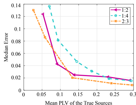
Figure 6: Median error vs. coupling strength (PLV) for different frequency ratios at SNR=-10 (dB) with two pairs of phase-phase coupled sources. The median errors decrease as the PLV of the simulated coupled oscillations increases. Even for weak couplings (e.g. PLV=0.1), the errors of pattern extraction are small.
