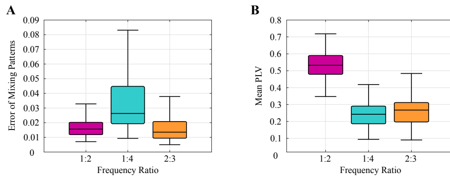
Figure 5: The performance of NID for extraction of five pairs of cross-frequency phase-phase coupled oscillations at SNR = -10 (dB) and different frequency ratios applied on simulated EEG. (a) Box-plots of error of mixing patterns. (b) Box-plots of the mean PLV. We conclude the reliable performance of NID from the small activation pattern errors and large mean PLVs.
