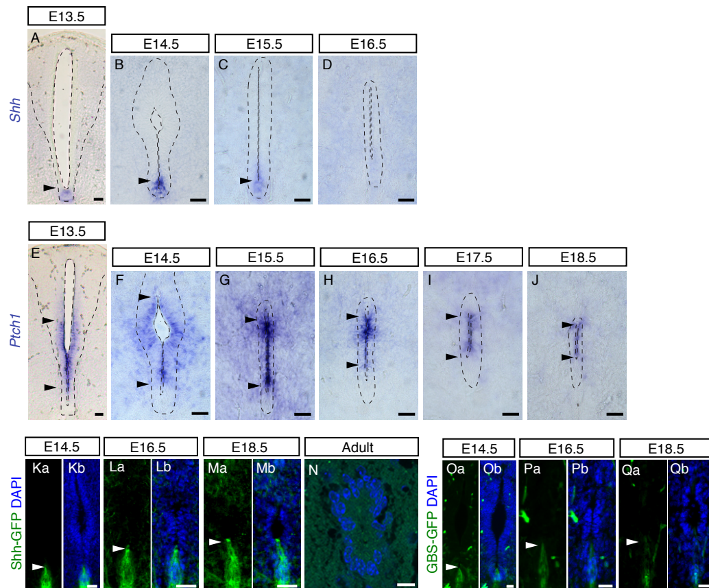
Figure 6 Shh activity persists after decline in Shh transcripts during mouse spinal cord development (A-D) In situ hybridisation showing Shh mRNA expression in the floor plate (arrowheads) at the indicated stages (E13.5: 14 sections, n = 3 embryos; E14.5: 15 sections, n = 5 embryos; E15.5: 58 sections/explants, n = 9 embryos; E16.5: 38 sections/explants, n = 9 embryos). From E17.5 onwards, Shh mRNA expression was no longer detected in the spinal cord (E17.5: 38 sections/explants, n = 8 embryos; E18.5: 18 sections, n = 3 embryos; 24- and 40-week-old: 17 sections, n = 3 adult mice; data not shown); (E-J) Ptch1 mRNA expression at the indicated stages (E13.5: 27 sections, n = 5 embryos; E14.5: 26 sections/explants, n = 5 embryos; E15.5: 43 sections/explants, n = 6 embryos; E16.5: 49 sections/explants, n = 8 embryos; E17.5: 40 sections/explants, n = 8 embryos; E18.5: 16 sections, n = 3 embryos). Note Ptch1 is excluded from the floor plate and detected in ventral half of the ventricular layer (between arrowheads) and persists in the forming central canal E18.5, but was no longer detected in adult (40-week-old: 24 sections, n = 3 mice; data not shown). (Ka-Mb) Immunofluorescence for GFP in Shh-GFP embryos was detected in the floor plate during development (arrowheads) E14.5: 17 sections, n = 1 embryo; E16.5: 17 sections, n = 1 embryo; E18.5: 18 sections, n = 1 embryo, (N) but not in adult central canal (9-10 week adult (88 sections, n = 3 mice); (Oa-Qb) Immunofluorescence for GFP (arrowheads) in GBS-GFP embryos revealed positive cells in the ventral region at indicated stages (E14.5: 47 sections, n = 3 embryos; E16.5: 43 sections, n = 3 embryos; E18.5: 33 sections, n = 3 embryo). Ka-Qb, nuclei are stained with DAPI (blue). All scale bars: 40 μm, except N: 10 μm.
