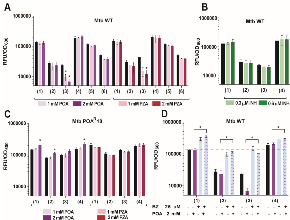
Figure 2. Effect of POA, PZA, INH treatment and POA/bortezomib co-treatment on levels of various RFP-PanD fusions.
