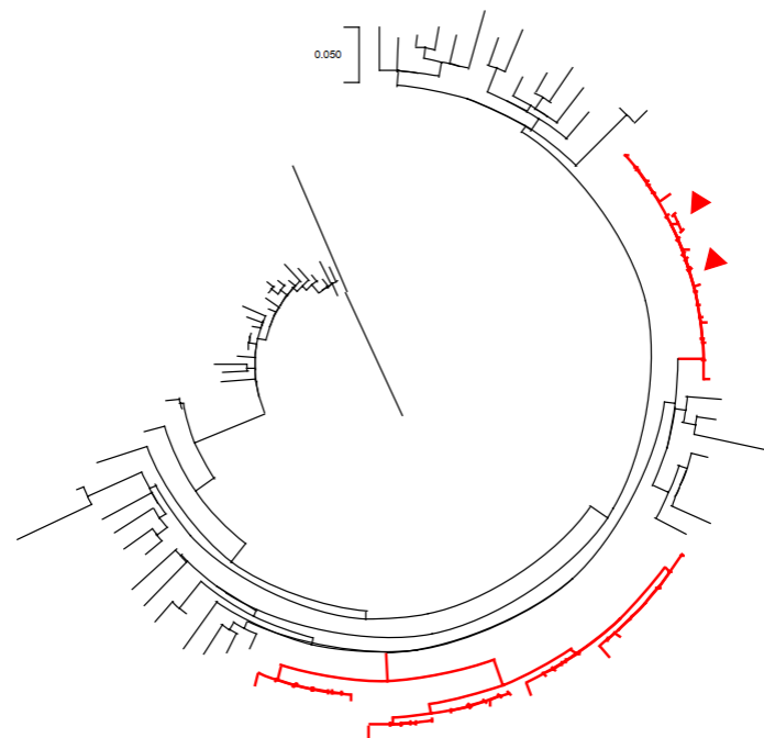
Figure 5 The phylogenetic tree to identify the FAW strains of collected from Yunnan, China. The red branched presented the C strain, the red triangles present the two Yunnan samples.
