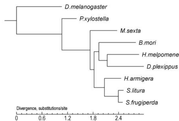
Figure 3 The phylogenetic relationships among nine lepidopteran genomes.
