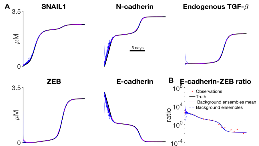
Fig 3. Data assimilation reconstructs unobserved EMT dynamics. (A) The truth (black), ensembles (blue), and ensemble mean (magenta) are shown as a function of time, for key epithelial and mesenchymal markers. (B) Observations (red stars) of the E-cadherin-ZEB ratio are shown for each observation interval \Delta t_{obs} . Parameters: Exogenous TGF\beta = 3 \mu M . Observation interval \Delta t_{obs} = 24 hours, number of ensembles k = 10 , multiplicative inflation \rho = 1 .
