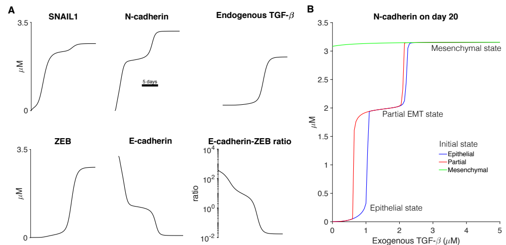
Fig 2. \text{TGF}\beta induces EMT via a partial or intermediate EMT state transition. (A) The time course of key epithelial and mesenchymal markers or a ratio of markers are shown as a function, following the addition of exogenous \text{TGF}\beta . (B) The expression level of N-cadherin on day 20 are shown as a function of the exogenous \text{TGF}\beta dose, for different initial conditions. The step-like response illustrates distinct cell states, corresponding with epithelial, partial or intermediate EMT, and mesenchymal states. Parameters: (A) Exogenous \text{TGF}\beta = 3 \mu\text{M} .
