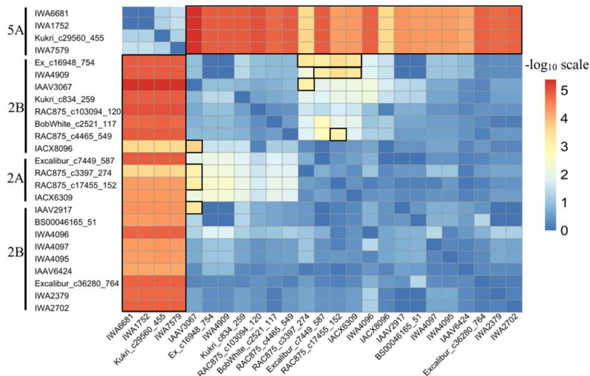
Figure 3: Heat map showing all possible pairwise epistatic interactions between the markers associated with vQTL on chromosomes 2A and 2B or mvQTL on chromosome 5A. Chromosome information of each marker is given on the left side. The heat map is sorted and color coded based on -\log_{10}(p\text{-value}) scale with the legend given on right side. Interactions that are significant ( -\log_{10}(p\text{-value}) > 3.8 ) are color coded as red or orange in color and outlined in black box.
