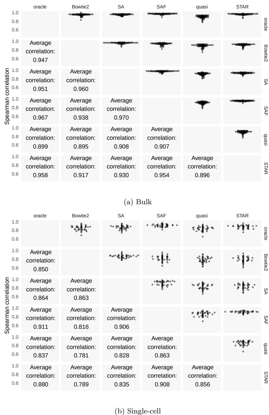
Figure 2: Performance of each method on real bulk and single-cell datasets. The top half of the matrix shows swarm plots of the pairwise correlations of the TPM values predicted by different approaches on the experimental samples. The bottom half shows the average Spearman correlation across the 109 bulk and single-cell samples.
