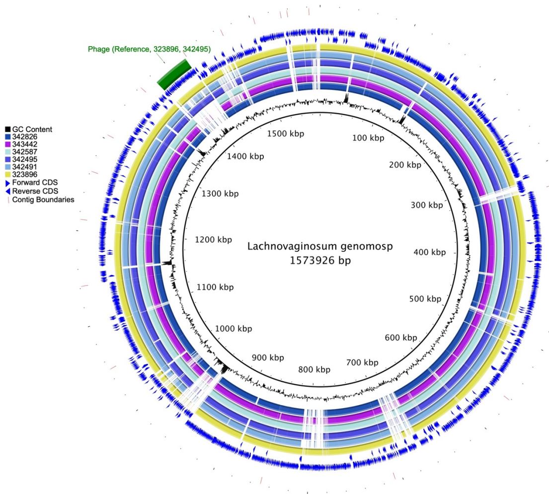
Figure 2. Circle plot comparing the Lachnovaginosum genomosp. metagenome-assembled genomes. The MAG sequenced on the Sequel II platform is the reference. Circles are from inside to outside: 1) genome size, 2) GC content, followed by MAGs 3) 342826 4) 343442, 5) 342587, 6) 342495, 7) 342491, 8) 323896 and finally 9) forward-direction coding sequences, 9) reverse-direction coding sequences, 10) phage detected in reference genome (green bar), and 11) contig boundaries for reference genome.
