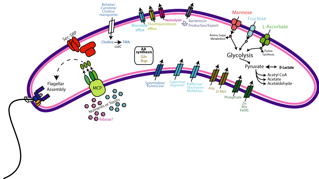
Figure 3. Genomic features of Lachnovaginosum genomospecies. Genes coding for the following functions were conserved across all genomes: Methyl-accepting chemotaxis (MCP) and subsequent flagella assembly, Sec-SRP secretion systems, choline import and metabolism, bacteriocin production and export, mannose, fructose, and L-ascorbate transport and metabolism, D-lactate dehydrogenase and biosynthesis of only 2 amino acids.
