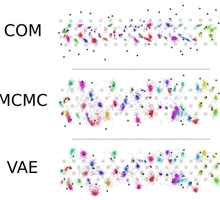
Figure 4: Estimated spike locations for the different methods on a 10 \mu V recording. Center of mass estimates (top) are calculated using 7 channels. The MCMC estimated locations (middle) used 8-14 channels of observed amplitudes for inference, and the VAE model (bottom) was trained on 8-14 channels surrounding each spike and 0 amplitude jitter (see 3.3.2 for amplitude jitter explanation).
