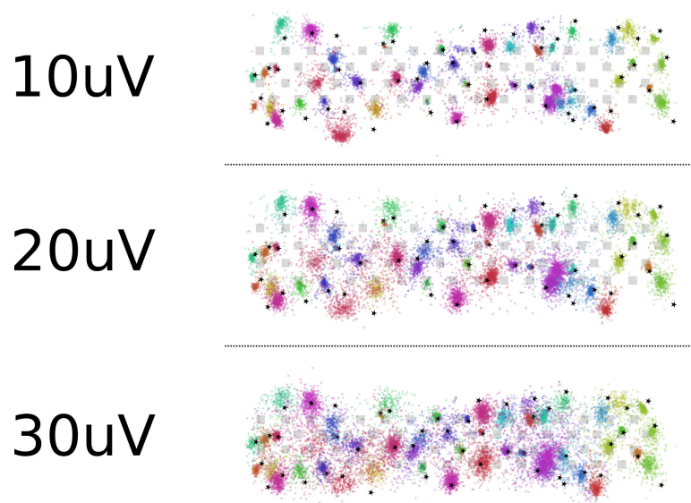
Figure 6: Effect of noise on location inference for the VAE on the Neuropixels probe . We vary the noise levels for the recording from 10μV, 20μV, and 30μV. Increasing the noise also increases the number of outliers in and the spread of the location estimates.
