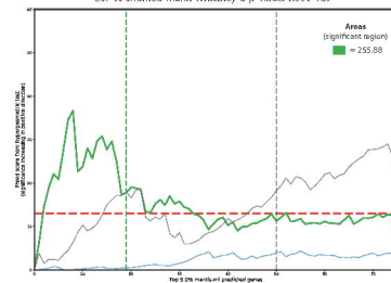
Random Forest LoF vs 'shuffled' Mann-Whitney-U p-value: 1.55e-189
