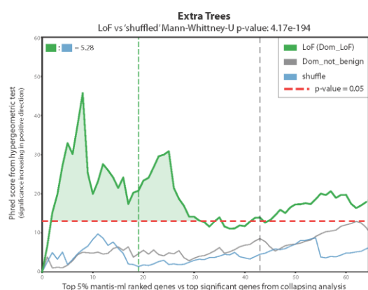
Fig. 4. Cross-validation of mantis-ml predictions with cohort-level rare-variant association studies. a) Hypergeometric test enrichment of disease-specific mantis-ml predictions with collapsing analysis results from CKD (i), Epilepsy (ii) and ALS (iii) cohorts. The horizontal dashed red line corresponds to the significance threshold
