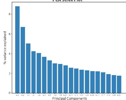
b. PCA Scree Plot
