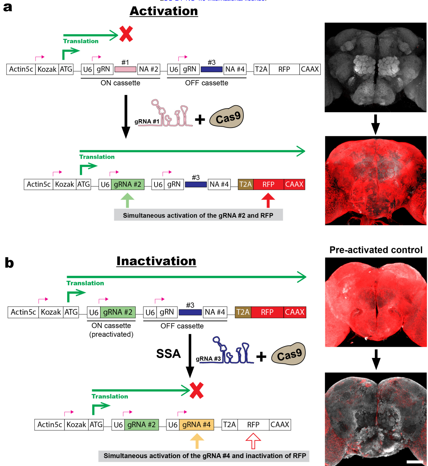
Fig 2. A coupled cascade of gRNAs and reporters
