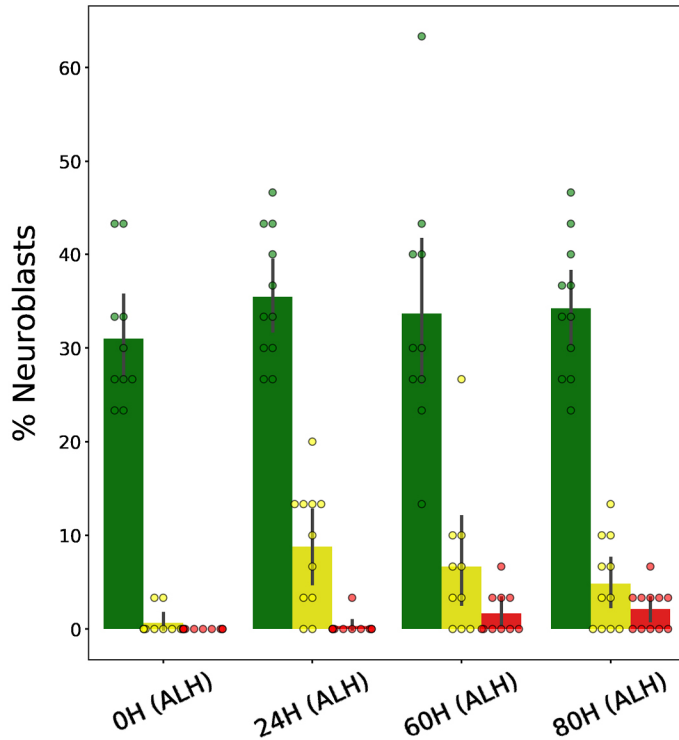
Fig. S8. CLADES 1.0 progression over the larval development.
