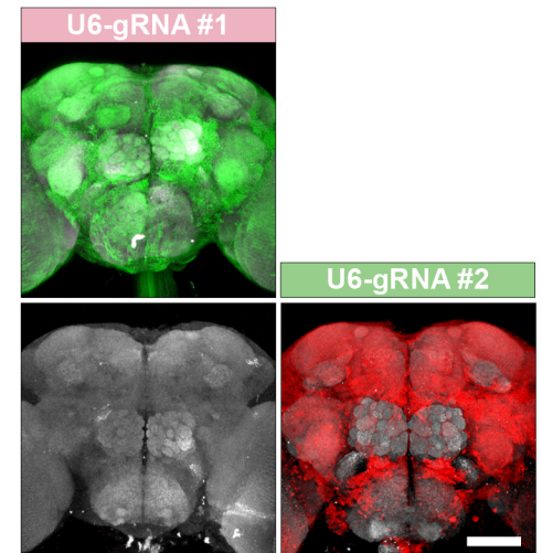
Fig. S7. CLADES 1.0 can only be activated by the combination of Cas9 and the trigger gRNA.
