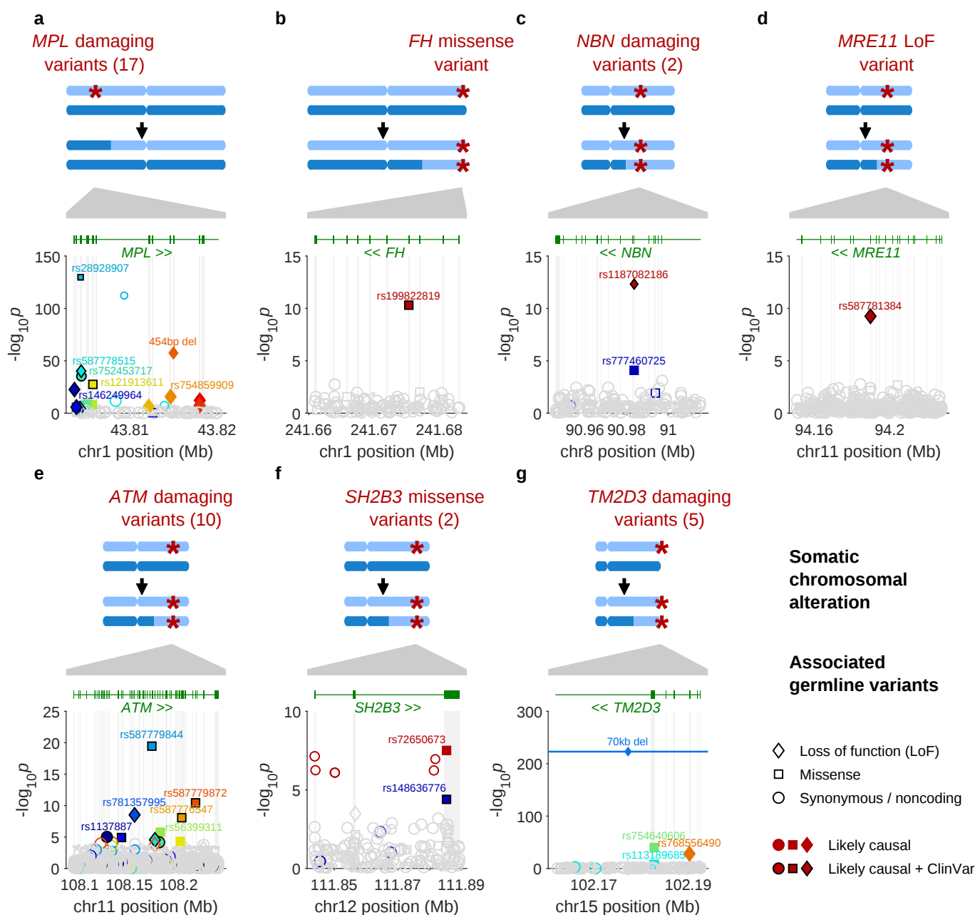
Figure 2. Fine-mapped inherited sequence alleles associated with the acquisition/selection of CNN-LOH mutations in cis. (a) MPL , (b) FH , (c) NBN , (d) MRE11 , (e) ATM , (f) SH2B3 , (g) TM2D3 . At each locus, the CNN-LOH mutations acquired by expanded clones tend to have deleted (a) or duplicated (b–g) the inherited alleles in a predictable manner as shown. Each panel is organized in the following way: top, genomic modifications observed in clones; bottom, association P -values (Fisher’s exact test) vs. chromosomal position. All variants with filled symbols are likely causal coding or splice variants (Table 1); black marker edges indicate evidence of pathogenicity in ClinVar [21]. Distinct colors are used to indicate the statistical independence of variants; any variants in linkage disequilibrium with likely causal variants ( R^2 > 0.2 in cases) are indicated with open symbols with a border color matching that of the likely causal variant. Symbol shapes indicate the effects of the indicated variant on encoded protein (LoF, missense, etc.); symbol sizes scale inversely with minor allele frequency.
