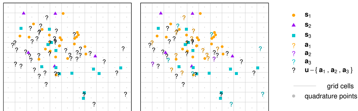
Figure 1: Three illustrative point patterns. The orange, purple, and turquoise colored dots represent locations with known species identity, s_1 , s_2 , and s_3 . The gray dots represent quadrature points q , which are spaced evenly along a regular grid such that one quadrature point is at the centre of each rectangular grid cell. The black question marks (left) represent observed locations u with uncertain species identity. The locations in a_1 \in u , a_2 \in u , and a_3 \in u which are reclassified as belonging to one of the species are represented by coloured question marks (right).
