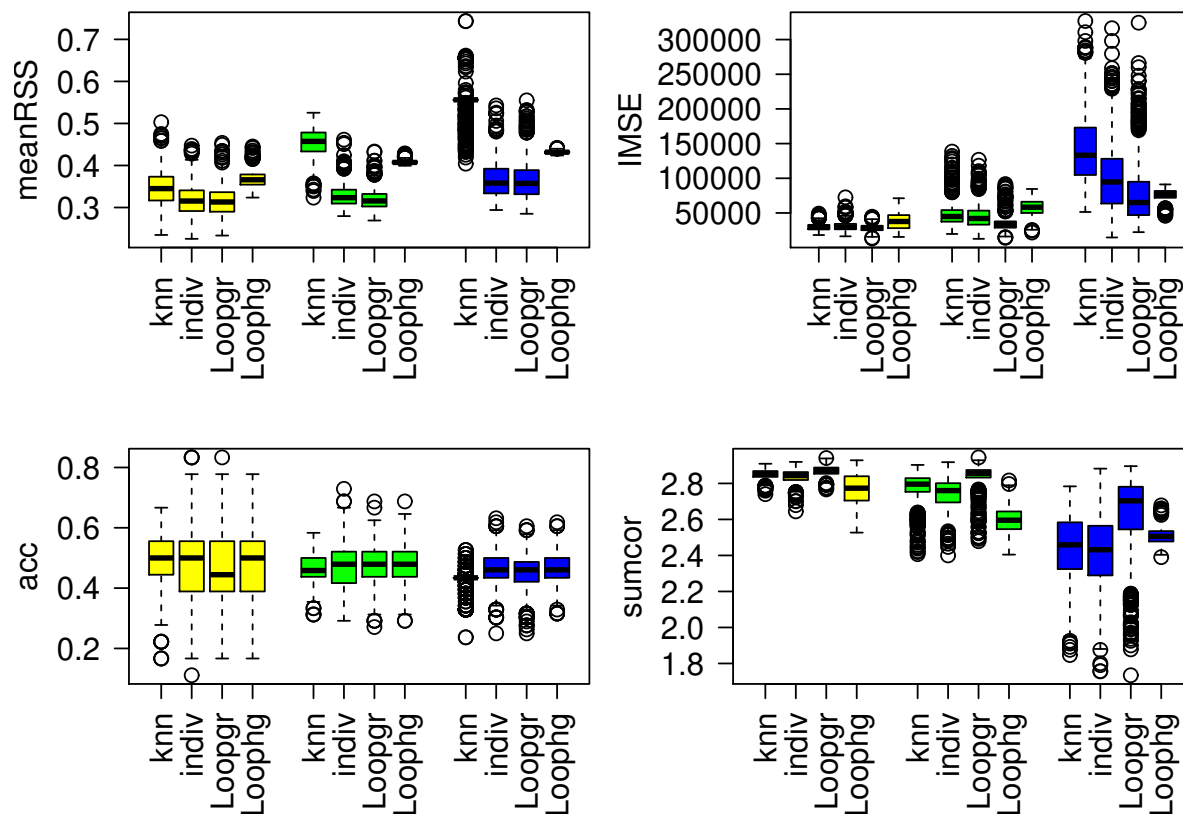
Figure 3: Measures of performance for the knn, individual, Loop grW and Loop hgW methods. Each color boxplot represents a different percentage of hidden observation: in yellow are the performances with 20% of hidden observations, in green with 50% and in blue with 80%. The parameters of abundances and correlation are: m_1 = 32 , m_2 = 42 , m_3 = 23 ; \rho_{1,2} = 0.85 , \rho_{1,3} = -0.09 , \rho_{2,3} = 0.20 .
