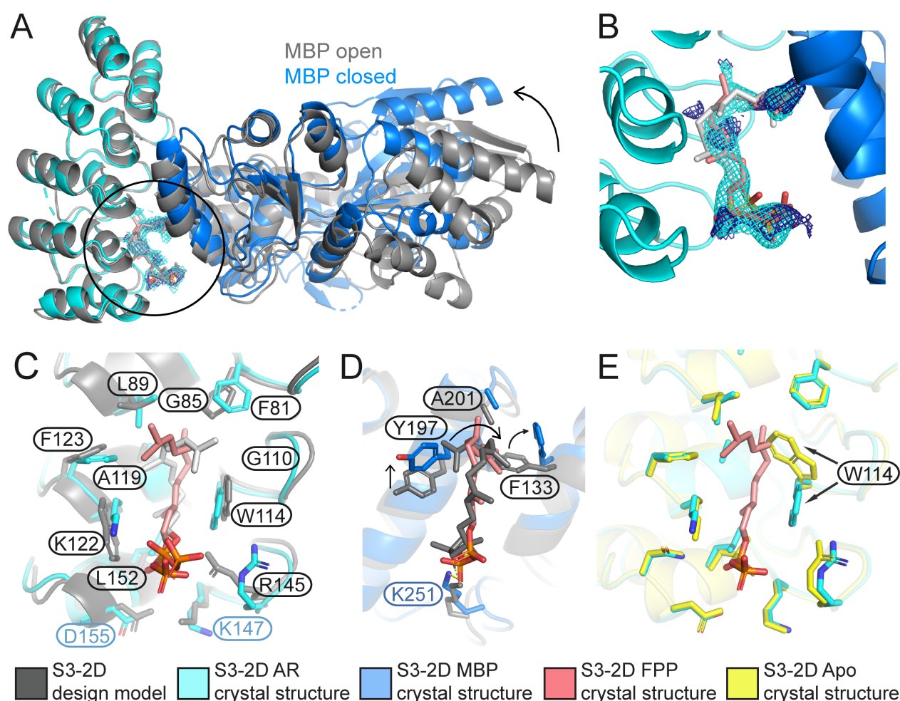
Fig. 4. The S3-2D crystal structure matches the computational design with atomic accuracy. (A) Overlay of the design model (grey) with the crystal structure (designed AR: cyan, designed MBP: blue, FPP: pink) showing FPP binding in the computationally designed binding site at the AR-MBP interface (circle). Note that the designs crystallized in the open MBP conformation while MBP was in the closed conformation in the original scaffold on which the model was based, leading to a difference in rigid-body orientation (arrow) of one lobe of MBP distal to the FPP binding site. (B) FPP overlaid with 2F_o - F_c electron density map ( 1.2\sigma , cyan) and ligand omit map ( 0.8\sigma , dark blue). Strong density peaks were present in both maps for the phosphates and several anchoring hydrophobic groups. (C) Open-book representation of FPP binding site on AR, showing close match of designed side chain conformations. (D) Open-book representation of FPP binding site on MBP, indicating a clash between the position of MBP Y197 in the crystal structure (blue) and the designed FPP orientation in the model (grey), causing slight rearrangements of FPP and F133 (arrows). (E) Alignment of the holo (cyan) and apo (yellow) structures of S3-2D, showing overall agreement with the exception of the side chain of W114 (arrows). In panels (C-E), residues are labeled black when designed and green/blue when present in the original scaffold complex.
