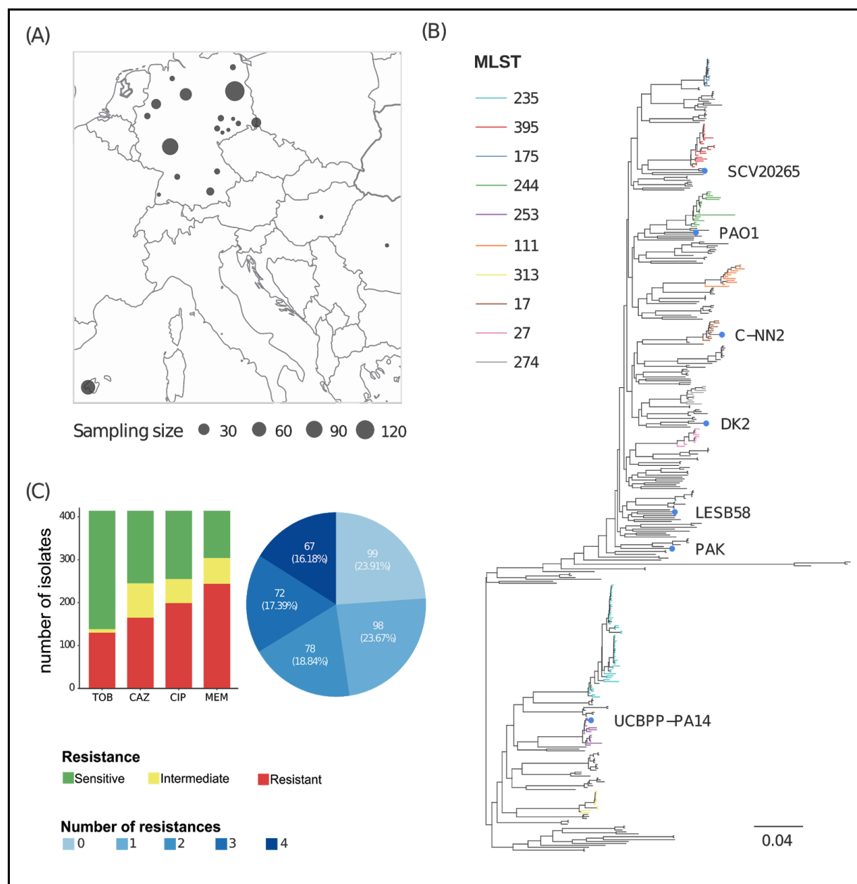
Figure 1: Geographic and phylogenetic distribution of 414 clinical P. aeruginosa isolates used in this study. (A) Geographic sampling site distribution, where circle size is proportional to the number of isolates from a particular location. (B) Phylogenetic tree of the clinical isolates and seven reference strains (a PA7-like outgroup clade including two clinical isolates is not shown). Abundant high risk clones identified by multi-locus sequence typing (MLST) are indicated by branch coloring. (C) Antimicrobial susceptibility profile
