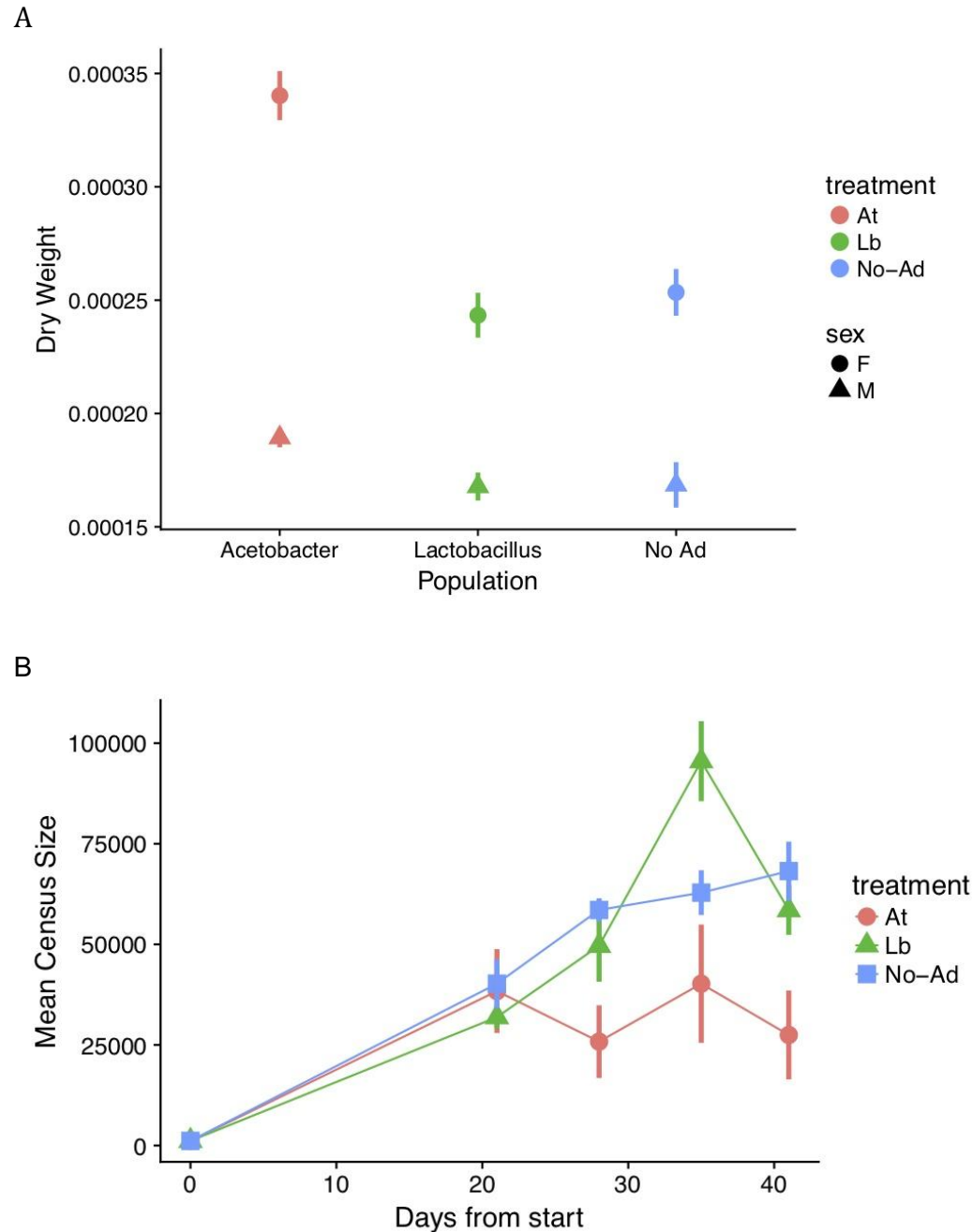
Figure 2: Population size and body mass of D. melanogaster populations from each microbial addition treatment. Panel A shows the mean from each treatment of the dry weight of D. melanogaster individuals of each sex from each replicate cage. Panel B shows host population size over the course of the experiment. Both panels values plotted are means \pm SEM.
