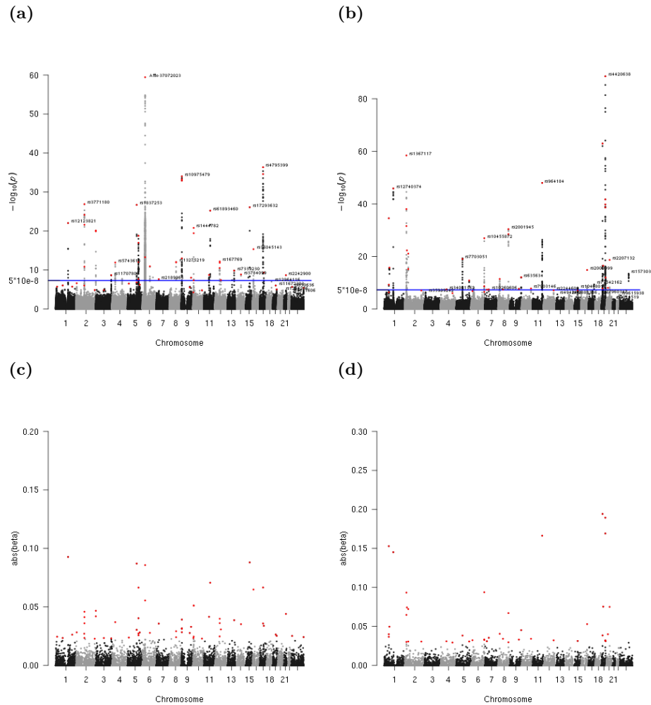
Figure 14: Manhattan plots of the univariate p -values and lasso coefficients for asthma (a, c) and high cholesterol (b, d). The vertical axis of the p -value plots shows -\log_{10}(p) for each SNP, while the vertical axis of the coefficient plots shows the magnitude of the coefficients from snpnet . The SNPs with relatively large lasso coefficients are highlighted in red. The blue horizontal line on the p -value plot represents a reference level of p = 5 \times 10^{-8} .
