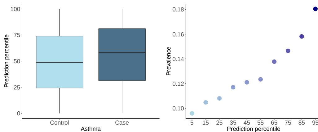
Figure 9: Results for asthma based on the best lasso model. Left: box plot of the percentile of the linear prediction score among cases versus controls. Right: the stratified prevalence across different percentile bins based on the predicted scores by the optimal lasso.
