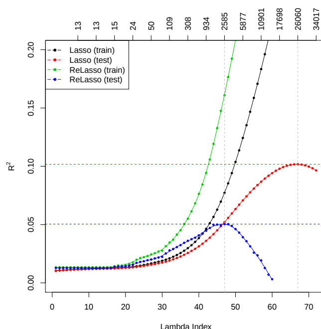
Figure 6: R^2 plot for BMI. The top axis shows the number of active variables in the model.
