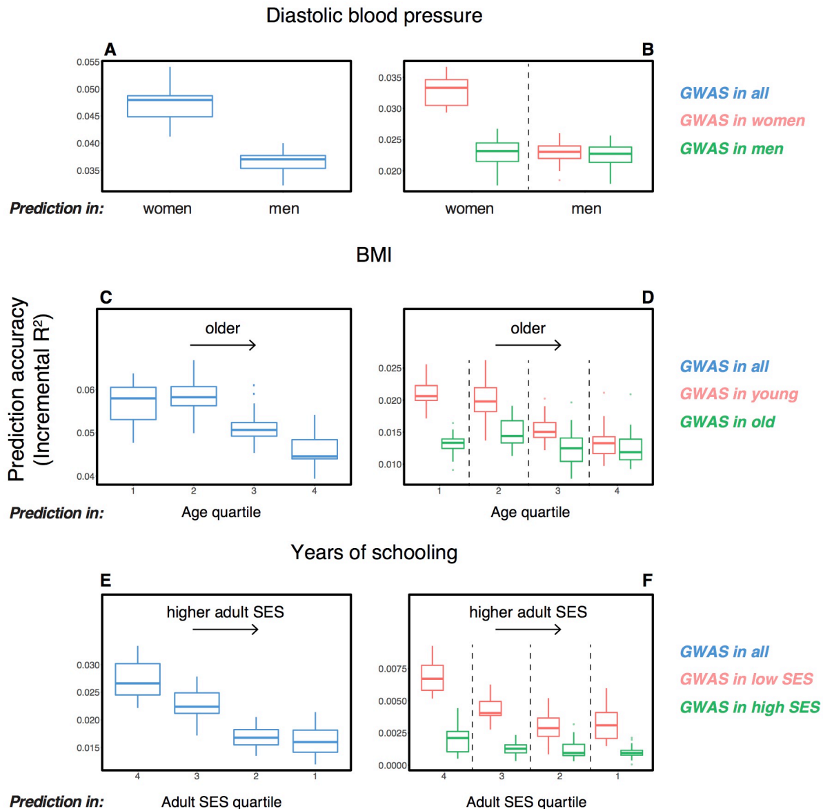
Figure 1: Variable prediction accuracy of polygenic scores within an ancestry group. Shown are incremental R^2 values (i.e., the increment in R^2 obtained by adding a polygenic score predictor to a model with covariates alone) in different prediction sets. Each box and whiskers plot is computed based on twenty choices of estimation and prediction sets. Thick horizontal lines denote the medians (A,C,E). The polygenic scores were estimated in large samples of unrelated WB individuals. Phenotypes were then predicted in distinct samples of unrelated WB individuals, stratified by sex (A), age (C) or Townsend deprivation index, a measure of SES (E). (B,D,F) Same as in A,C,E, but here the polygenic scores are based on a GWAS in a sample limited to one sex, age or SES group. When the GWAS is performed in the group that showed higher prediction accuracy in A,C,E (women, young, low SES), the qualitative trend is the same; but when the GWAS is performed in men, old or high SES, prediction accuracy is diminished and similar across groups.
