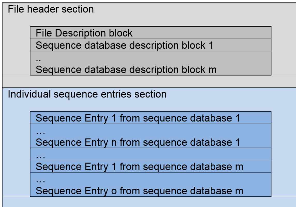
Figure 1. Overview of the PEF schema. The file header section encodes metadata about the file itself and about the one or more sequence databases contained in the file. The individual sequence entries section encodes each of the individual sequences and the metadata associated with each entry.
