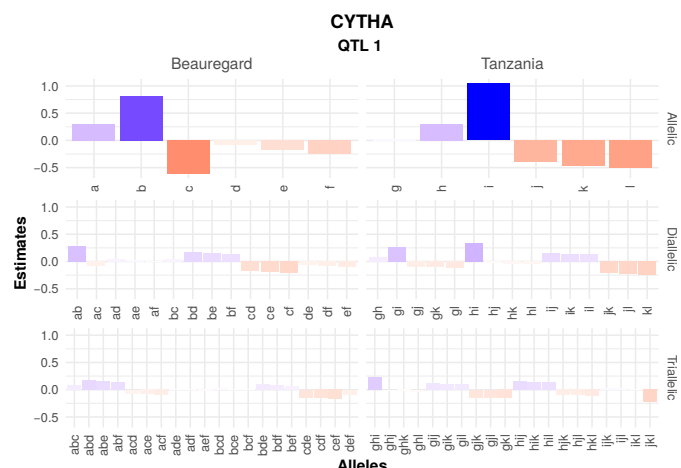
Figure 4 Allele and allele combination additive effects from the decomposed best linear unbiased predictions (BLUPs) for the QTL 1 (on linkage group 15 at 5.27 cM) of commercial root yield in t \cdot ha^{-1} (CYTHA) in a hexaploid sweetpotato full-sib family ('Beauregard' × 'Tanzania'). Marker-assisted selection for increasing CYTHA would have to focus on selection for alleles b and i , and against alleles c and j through l from the respective parents.
