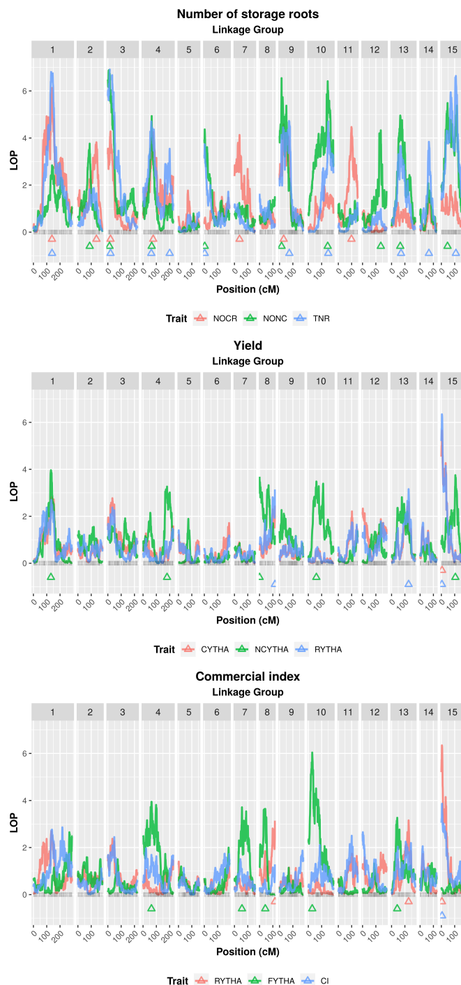
Figure 3 Logarithm of p -value (LOP) profiles from random-effect multiple interval mapping (REMIM) of eight yield-related traits from 'Beauregard' \times 'Tanzania' (BT) full-sib family. Triangles show the QTL peak location. Trait abbreviations: number of commercial (NOCR), noncommercial (NONC) and total (TNR) roots per plant, commercial (CYTHA), noncommercial (NCYTHA) and total (RYTHA) root yield in t \cdot ha^{-1} , foliage yield (FYTHA) in t \cdot ha^{-1} , and commercial index (CI).
