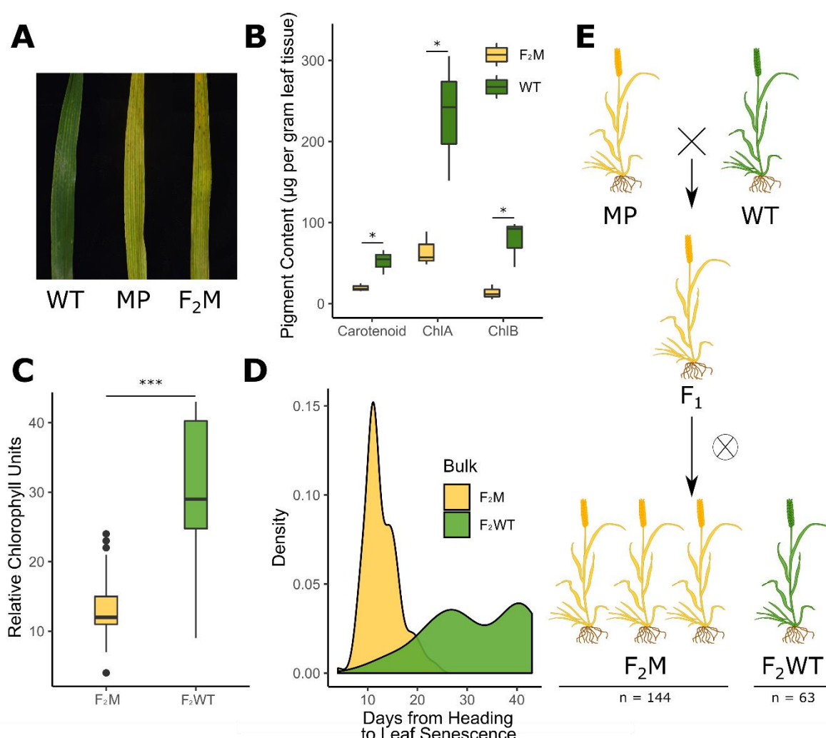
Figure 1: A premature yellowing phenotype from the Kronos TILLING population segregates as a single dominant locus. F 2 populations of the K2282 Kronos TILLING line grown at the JIC in 2016 showed an early yellowing phenotype (A). Pigment content was measured in the yellow mutant plants (F 2 M) compared to the wild-type plants (F 2 WT) (B; n = 3 per genotype) and was also quantified using SPAD (C; n = 153 F 2 M, n = 61 F 2 WT). The yellow group (F 2 M) senesced significantly earlier than the late bulk (F 2 WT) (D; n = 148 F 2 M, n = 56 F 2 WT). Scoring of the plants demonstrated that the F 2 population was segregating 3:1 for the yellow trait, indicative of a dominant single locus (E; numbers are combined for both populations). F 2 M and F 2 WT refer to plants which are yellow and green, respectively, and which derive from the F 2 population (see bottom of E), while WT and MP refer to Kronos WT plants or M 4 K2282 plants, respectively (see top of E).
