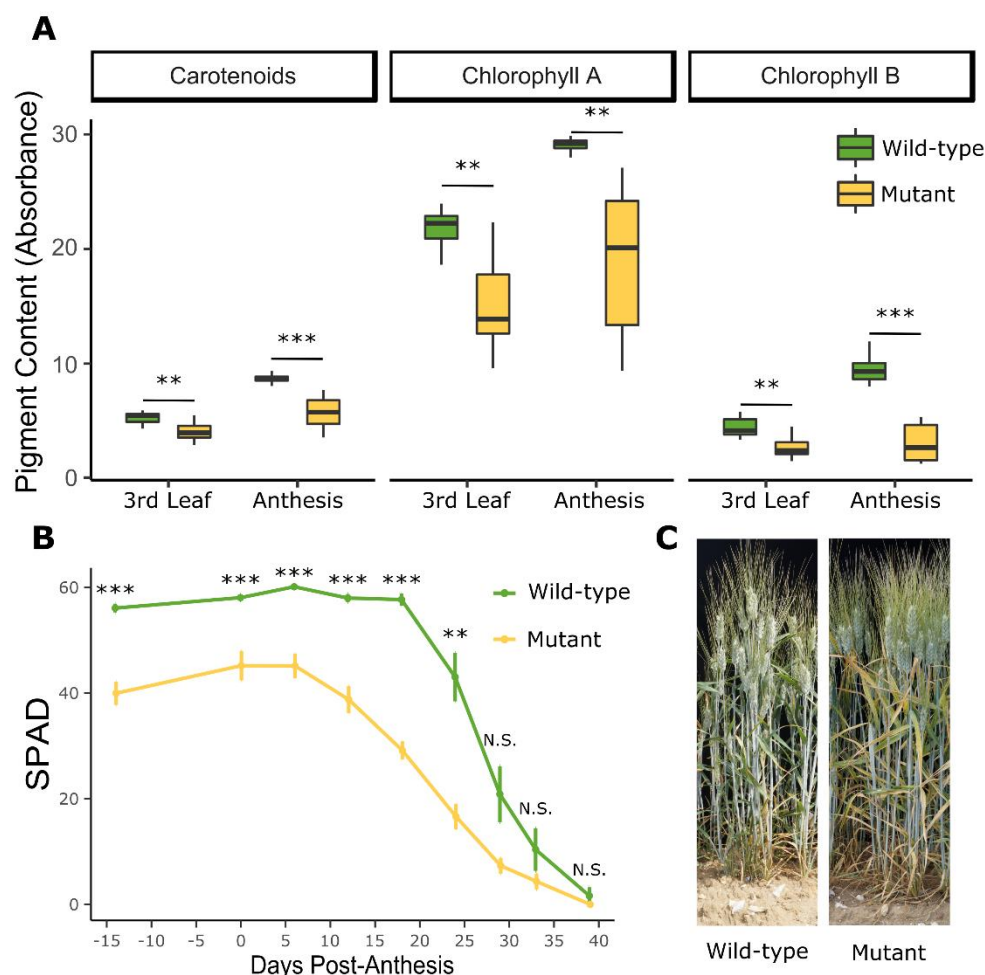
Figure 3: The YES-1 locus causes lower chlorophyll levels before anthesis and earlier onset of senescence. The early chlorosis phenotype was recapitulated in the JIC 2018 field trials.
