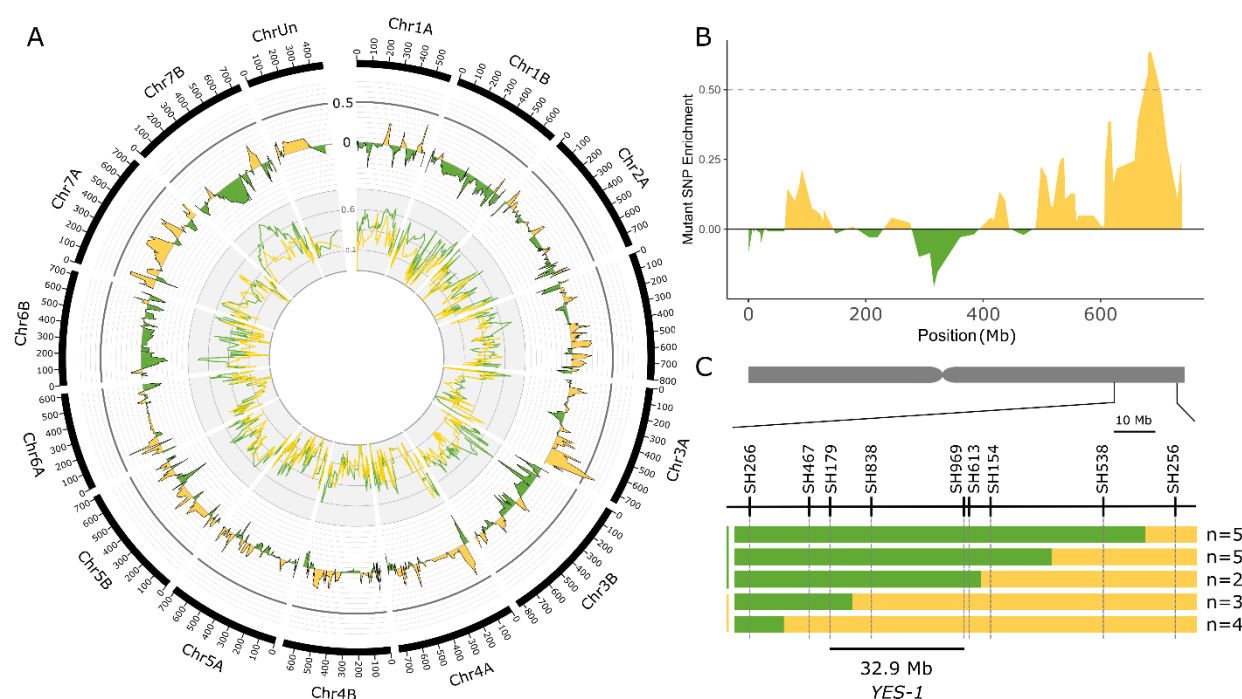
Figure 2: Bulked segregant analysis identifies the YES-1 locus on chromosome 3A. Exome capture was carried out on yellow and green bulks from K2282 x Kronos F 2 populations grown at the JIC in 2016. The K2282 yellow bulk (yellow line, inner track; smoothed to a moving average of 4) and green bulk (green line) were scored at each SNP locus identified for enrichment of the mutant allele. The level of enrichment in the green bulk was subtracted from that of the yellow bulk to obtain the \Delta value (outer track; smoothed to a moving average of 4). A high \Delta value, indicative of a region enriched for mutant alleles within the yellow bulks, was identified on the long arm of chromosome 3A (B; smoothed to a moving average of 4). Markers designed on known TILLING SNPs within this region mapped the YES-1 locus to a 32.9 Mb interval within the F 2 population (C). Green bars indicate wild-type calls, while yellow bars indicate mutant or heterozygous calls. The numbers of individual plants that fell into each recombination interval are shown to the right. The chromosome scale in (A) is given in Mb.
