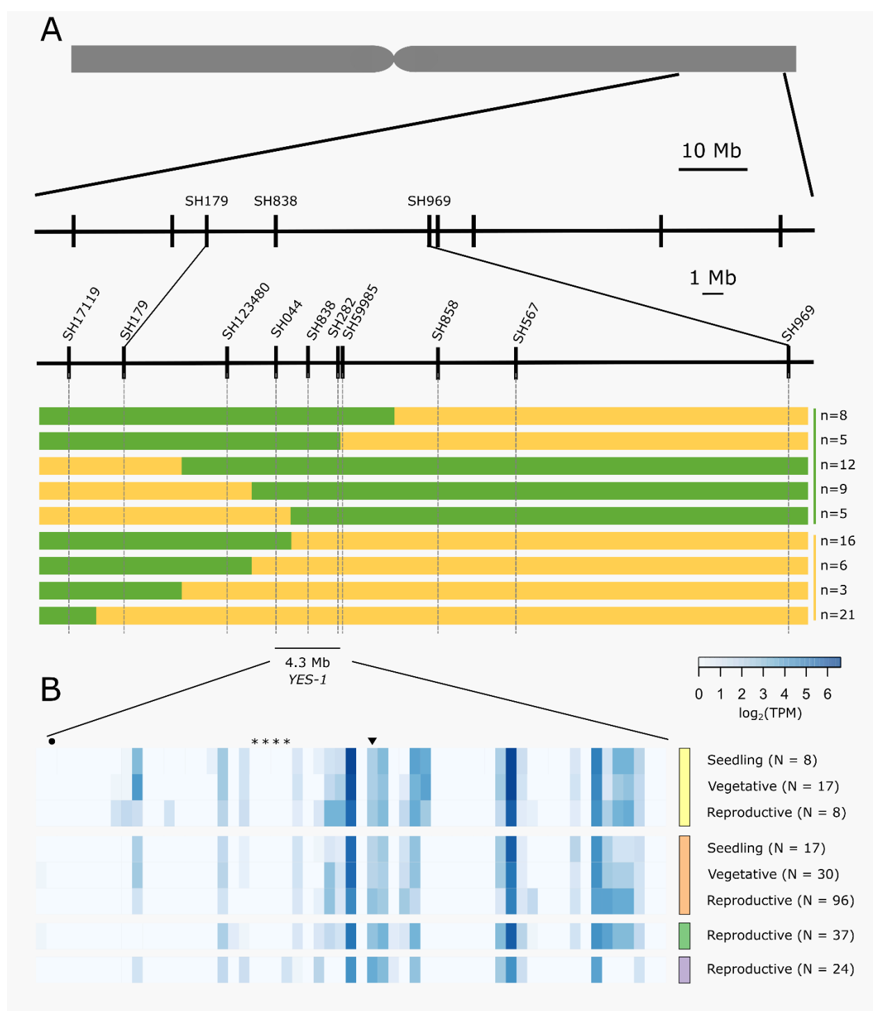
Figure 4: The YES-1 locus fine-maps to a 4.3 Mb region containing 59 genes. Markers were developed for novel SNPs identified in non-coding regions. We used phenotypic data from JIC 2017 and 2018 field trials to classify recombinant lines as green or yellow. (A). These markers mapped YES-1 to a 4.3 Mb interval between markers SH044 and SH59985. Expression data for the 59 high-confidence genes in the region (B) from developmental time course data (Ramírez-González et al., 2018) highlights gene expression in root (yellow, top), leaf/shoot (orange, second from top), spike (green, second from bottom) and grain (purple, bottom) tissues across developmental stages. Genes mentioned in the text are highlighted by an asterisk (TraesCS3A02G412900 to TraesCS3A02G413200; OsSAG12 orthologs), a circle (TraesCS3A02G410800; Tryptophan Decarboxylase 2 ) or an inverted triangle (TraesCS3A02G414000; putative magnesium transporter).
