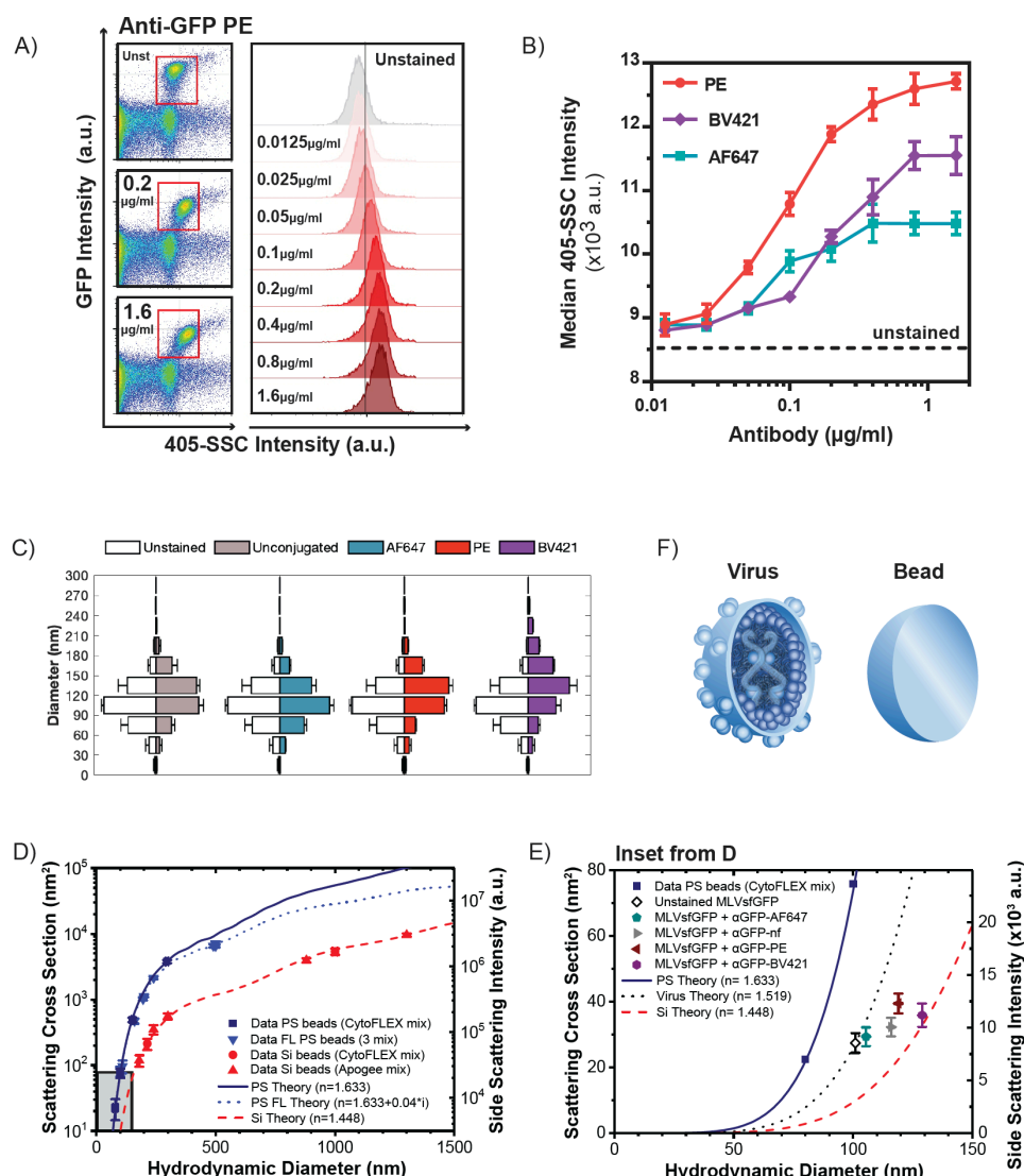
FIGURE 5. Antibody-fluorophore conjugates impact SSC intensity, hydrodynamic diameter, and effective refractive index of labeled viruses. (A) Antibody labeling of MLVsfGFP increases the SSC intensity of virus particles in a concentration-dependent manner. Representative scatter plots of MLVsfGFP (gated) mixed with MLVnoGFP that were unstained (Unst) or labeled with anti-GFP PE antibody at 0.2 \mu\text{g/ml} and 1.6 \mu\text{g/ml} (left panels). Histogram overlay of the gated GFP + populations that were labeled with anti-GFP PE, for all antibody concentrations from 0.0125 \mu\text{g/ml} to 1.6 \mu\text{g/ml} (right panel). (B) SSC intensity of GFP + viruses labeled with anti-GFP conjugated with PE, BV421, and AF647 at increasing antibody concentrations. Dashed line denotes SSC intensity of unlabelled MLVsfGFP. (C) NTA-measured diameter distribution of unlabelled MLVsfGFP separately compared to MLVsfGFP labeled with unconjugated anti-GFP, anti-GFP-PE, BV421, or AF647 at a concentration of 1.6 \mu\text{g/ml} ; n=3 . (D) Mie-theory analysis for the calculation of the RIs for data points acquired using different silica (Si; red) and polystyrene (PS; blue) beads. The plot represents a correlation of the scattering cross section, hydrodynamic diameter, and SSC intensity of the virus particles. The gray-shaded box indicates the range where the MLV data points were acquired. (E) Gray-shaded box inset from (D), Mie-theory analysis of unlabelled MLVsfGFP and viruses labeled with various anti-GFP conjugated antibodies. The estimated effective RI of unlabelled virus is demonstrated as a dotted black line; n=3 . (F) Cartoon to illustrate the complex and heterogeneous composition of a virus compared to the homogenous composition of a bead.
