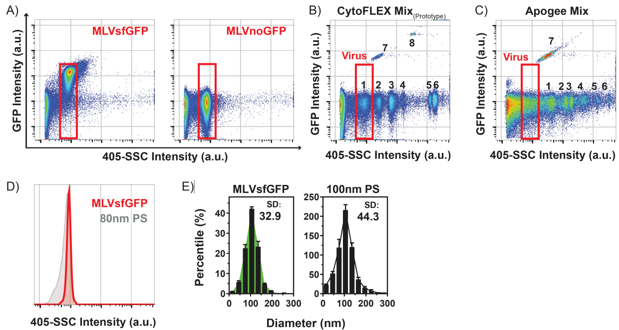
FIGURE 1. MLV virions are highly monodisperse. (A) MLVsGFP and MLVnoGFP virions are a discrete population that can be resolved by 405-SSC intensity (a.u.) and green fluorescence intensity (a.u.). (B) Prototype CytoFLEX Sizing Mix (1: 80 nm PS, 2: 100 nm PS, 3: 214 nm Si, 4: 152nm PS, 5: 296 nm PS, 6: 1020 nm Si, 7: 100 nm PS fluorescent, 8: 196 nm PS fluorescent) and (C) ApogeeMix (1: 180 nm Si, 2: 240 nm Si, 3: 300 nm Si, 4: 590 nm Si, 5: 880 nm Si, 6: 1300 nm Si, 7: 110nm PS fluorescent) were analysed using the same settings as those for the MLV viruses. The “Virus” gate in red is the same from panel A. (D) Comparison of the 405-SSC intensity (a.u.) of MLVsGFP and 80 nm polystyrene (PS) beads. (E) NTA on the diameter distribution of 100 nm PS beads and MLVsGFP; SD: standard deviation.
