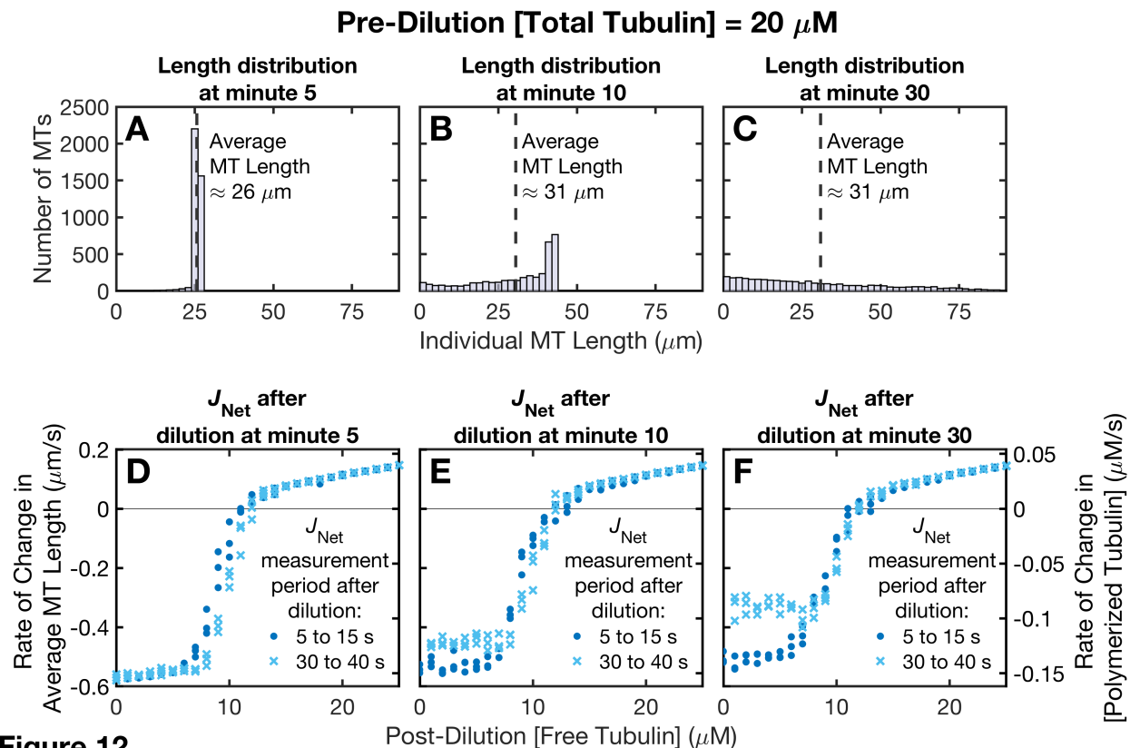
Figure 12: Effect on J_{\text{Net}} of varying the time at which the dilution is performed. Pre-dilution [total tubulin] = 20 \mu\text{M} . ( A,B,C ) Histograms of MT lengths at the time of the dilution: minute 5 (panel A ), minute 10 (panel B ), and minute 30 (panel C ) of the simulation. Note that panel A is before the system has reached polymer-mass steady state and that panels B-C are after the system has reached polymer-mass steady state, which is when the average MT length is no longer changing over time but the length distribution can still change. ( D,E,F ) J_{\text{Net}} measured from 5 to 15 seconds after the dilution and 30 to 40 seconds after the dilution (as indicated in the keys on the plots), for each of the three different dilution times: minute 5 (panel D ), minute 10 (panel E ), and minute 30 (panel F ). Methods: In panels A-C , the three independent replicates of the simulations are aggregated in each histogram. For each post-dilution [free tubulin], the conditions up to the time of dilution are the same. Therefore, for the histograms, we aggregated the MTs that will be diluted into the different post-dilution [free tubulin]: N = 3900 = (50 \text{ MT seeds per post-dilution [free tubulin] per replicate}) * (26 \text{ values of post-dilution [free tubulin]}) * (3 \text{ replicates}) . In panels D-F , data points are plotted for each of three independent replicates of the simulations at each value of post-dilution [free tubulin]. Interpretations: The later the dilution time (i.e., the longer the amount of time that the MTs are allowed to compete before the dilution is performed), the more short MTs are present at the time of the dilution (compare across panels A-C ). The shorter the MTs are at the time of the dilution, the sooner they undergo complete depolymerization after the dilution for low post-dilution [free tubulin] (see Figure 13 ). These complete depolymerizations cause the lower arm of J to shift upwards (compare across panels D-F ).
