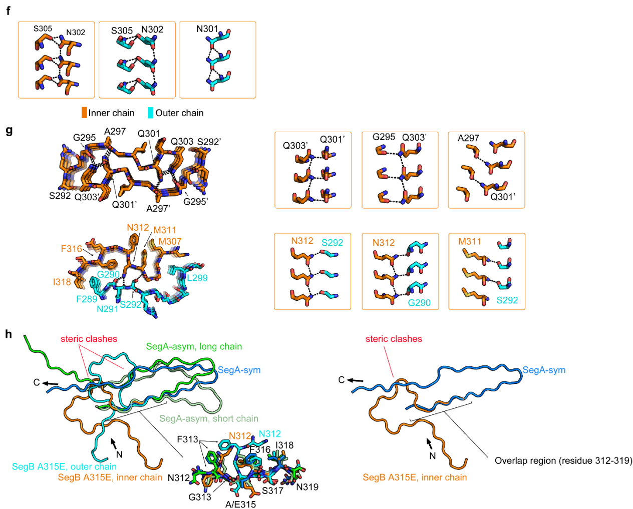
Supplementary Figure 5 Detailed analysis in TDP-43 fibril structures. f, Side view of hydrophilic interactions in the head of the R-shaped fold in the SegB A315E. g, (Left column, from top to bottom) Cross-section of three layers of the homodimer and heterodimer interfaces in SegB A315E are shown. Side view of the detailed interactions of each interface are shown in the right columns. h, Superposition of SegA and SegB A315E main chain models shows TDP-43 cannot simultaneously form a dagger-shaped fibril and an R-shaped fibril because of steric clashes; it must form either one or other. The simplified comparison using only SegA-sym to represent the dagger-shaped fold and SegB A315E inner chain to represent the R-shaped fold are showing on the right panel. Color coding in this figure is the same as in Figure 2 and 3, hydrogen bonds are shown as black dashed lines with distance between 2.3-3.2 Å. Detailed alignment parameters are listed in Supplementary Table 2.
