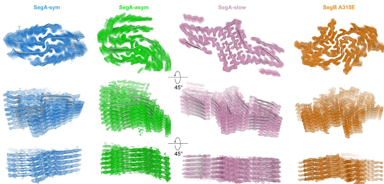
Supplementary Figure 4 Density maps of TDP-43 fibril structures. Different views of the four structures reported in this study, with 5 layers of each structure shown. Density maps are shown in colored mesh and atomic model are shown in grey cartoons. Top-views demonstrate clear separation of beta-strands while tilted views demonstrate clear separation of the beta-sheets in the z-direction.
