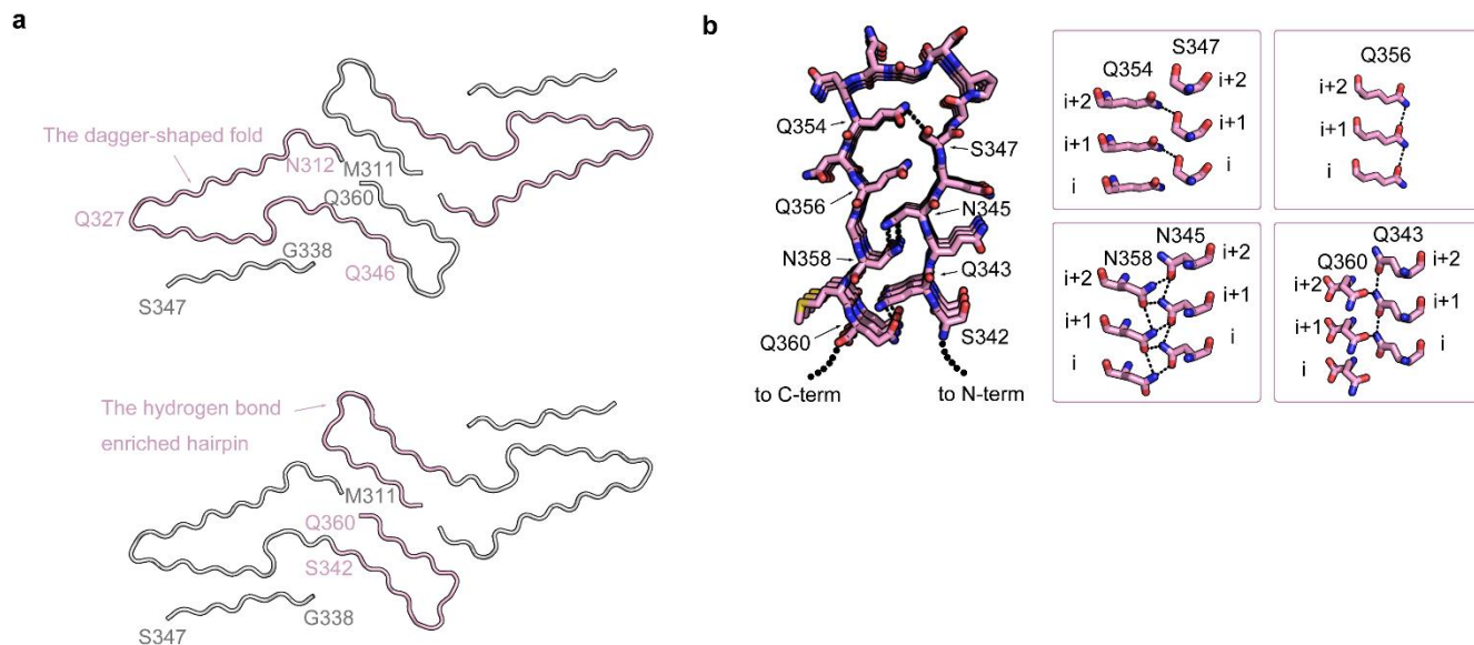
Supplementary Figure 8 The dagger-shaped fold and the hydrogen bond enriched hairpin structure in SegA-slow. a , SegA-slow is shown in cartoon. The dagger-shaped fold (residue 312-346, upper panel) and the hydrogen bond enriched hairpin (residue 342-360, bottom panel) is colored pink, and the rest of the residues are colored gray. Note that both the dagger-shaped fold and the hydrogen bond enriched hairpin are individually compatible with full-length TDP-43 with free N- and C-terminals. b , Top view of hydrogen bond enriched hairpin structure in SegA-slow (left) and (right) side views of residues involved in hydrogen bond network.
