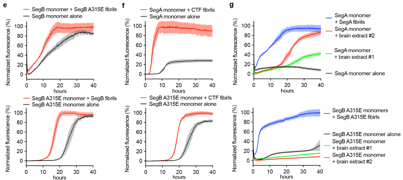
Supplementary Figure 1e-gThT seeding assays of TDP-43 segments. ThT aggregation curves of TDP-43 segments with or without seeding. Data are shown as mean \pm s.d., n=4 independent experiments.
