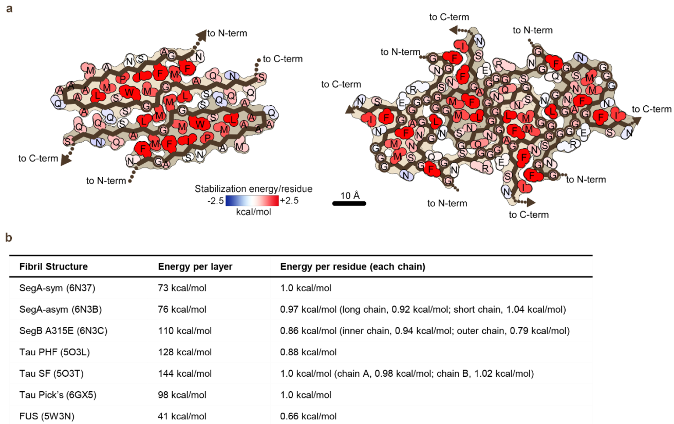
Figure 3 Calculated solvation energy maps for TDP-43 fibrils based on atomic solvation
