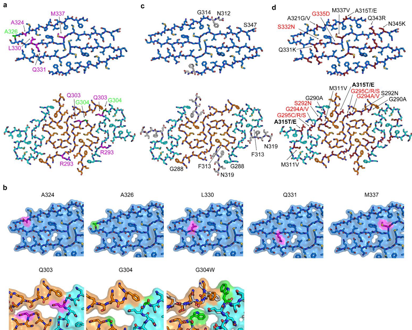
Supplementary Figure 6 Mutation analysis of TDP-43 fibril structures. a & b , Residues tested in mutagenesis study in (top) SegA-sym and (bottom) SegB A315E. Residues that reduce pathological fragment TDP-CTF aggregation when mutated are shown in magenta and those that do not influence TDP-CTF aggregation when mutated are shown in green. Arg293 was mutated to glutamate and others were mutated to tryptophan. In (b), the models of both structures are shown in sticks and semitransparent surface mode. Notice that Ala324, Leu330, Gln331 and Met337 in SegA-sym and Gln303 in SegB A315E (also see Supplementary Figure 7) are in a tightly packed environment that does not tolerate a tryptophan mutation, consistent with our previous mutagenesis study where these mutations delayed the aggregation of the pathogenic TDP-43 fragment.
