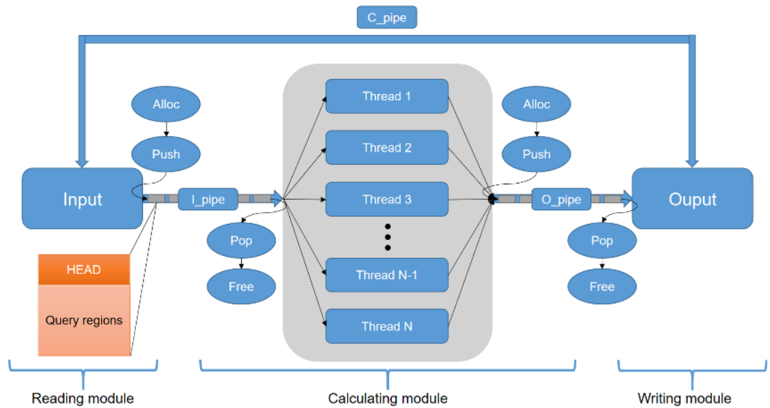
422 423 Figure 5 The multithreaded program for efficiently annotating openness of a 424 vast amount of genomic regions
