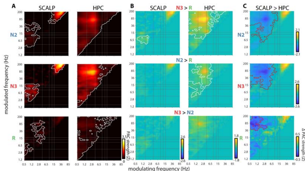
Figure 5. Group-level phase-amplitude coupling. (A) Mean coupling strength for scalp (left) and HPC (right). White outlines indicate clusters of significantly greater than zero coupling ( P<0.05 , cluster-based permutation test). (B) Mean difference in coupling strength between sleep stages for scalp (left) and HPC (right). (C) Difference in coupling strength between scalp and HPC. White/red outlines in (B) and (C) indicate significant positive/negative clusters, respectively ( P<0.05 , cluster-based permutation test).
