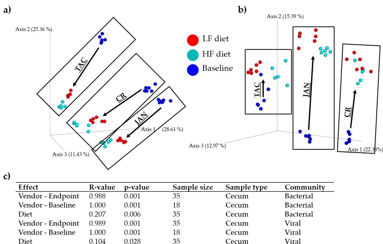
Figure 3. Bray Curtis dissimilarity metric PCoA based plots of a) the caecal bacterial community and b) viral community at baseline (5 weeks of age) and after 13 weeks on low fat or high diet (18 weeks of age), respectively. c) ANOSIM of the Bray Curtis distances of the effects of diet and vendor at baseline and endpoint (18 weeks of age). CR = Charles River, JAN = Janvier, TAC = Taconic. Black boxes frame the samples associated to the mice vendor.
