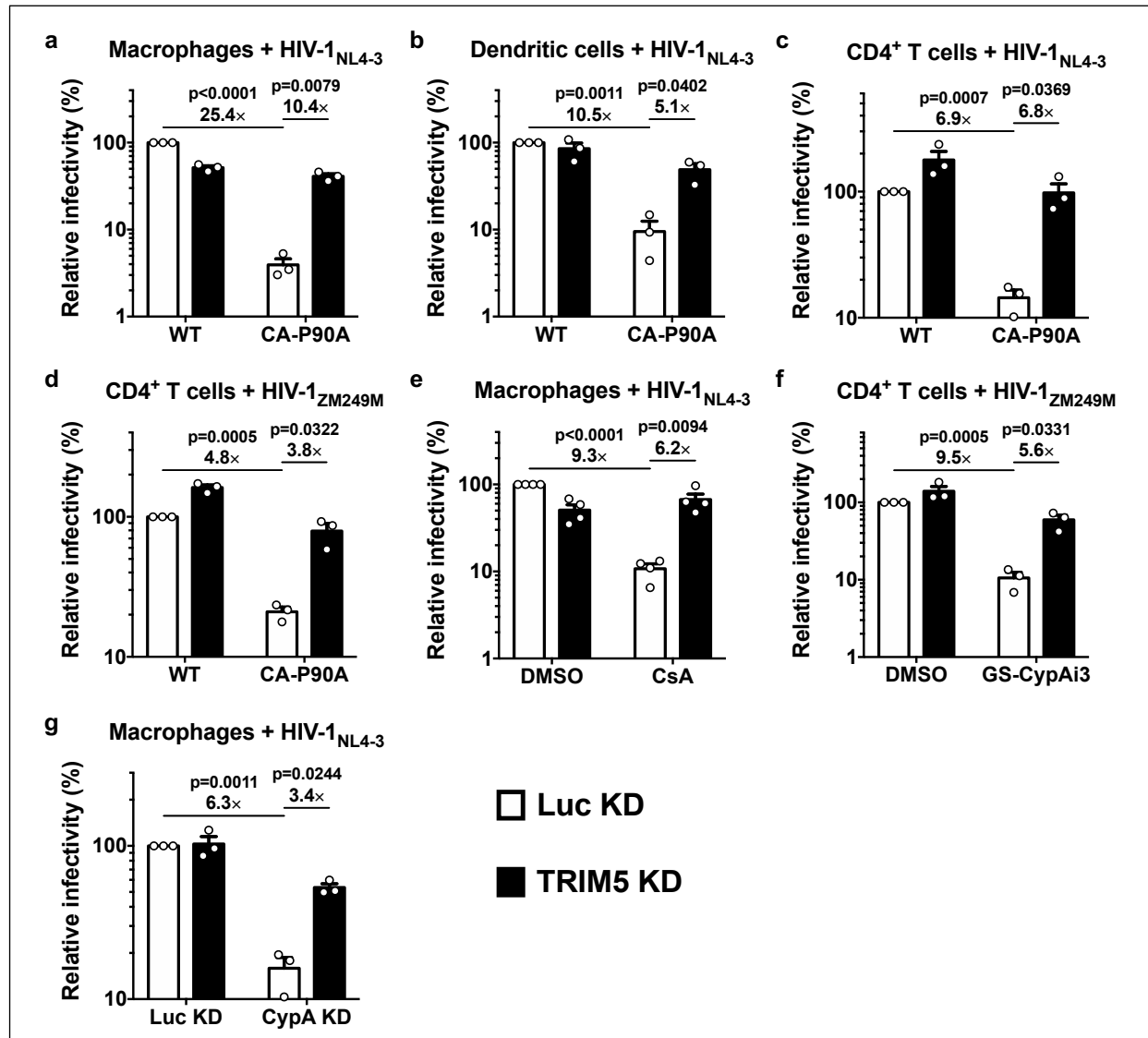
Fig. 1. Disruption of the CA-CypA interaction in primary human blood cells renders HIV-1 susceptible to restriction by TRIM5. a, Macrophages, b, dendritic cells, or c and d, CD4 + T cells, were selected after transduction with a lentivirus expressing shRNA targeting TRIM5 or Luc control, and challenged with single-cycle, VSV G-pseudotyped, HIV-1 NL4-3 GFP (a-c) or HIV-1 ZM249M GFP (d), bearing WT CA or CA-P90A (mean ± SEM, n = 3 donors for each). e, TRIM5 knockdown or Luc knockdown macrophages were challenged with HIV-1 NL4-3 GFP in the presence of 8 μM CsA or DMSO solvent (mean ± SEM, n = 4 donors). f, TRIM5 knockdown or Luc knockdown CD4 + T cells were challenged with HIV-1 ZM249M GFP in the presence of 2.5 μM GS-CypAi3 or DMSO solvent (mean ± SEM, n = 3 donors). g, Macrophages were transduced simultaneously with two vectors expressing shRNAs, as indicated, and selected with puromycin and blasticidin. Cells were then challenged with HIV-1 NL4-3 GFP (mean ± SEM, n = 3 donors). The percentage of GFP + cells was assessed by flow cytometry and normalized to WT in Luc control knockdown cells in all cases. Significance was determined by two-tailed, paired t-test.
