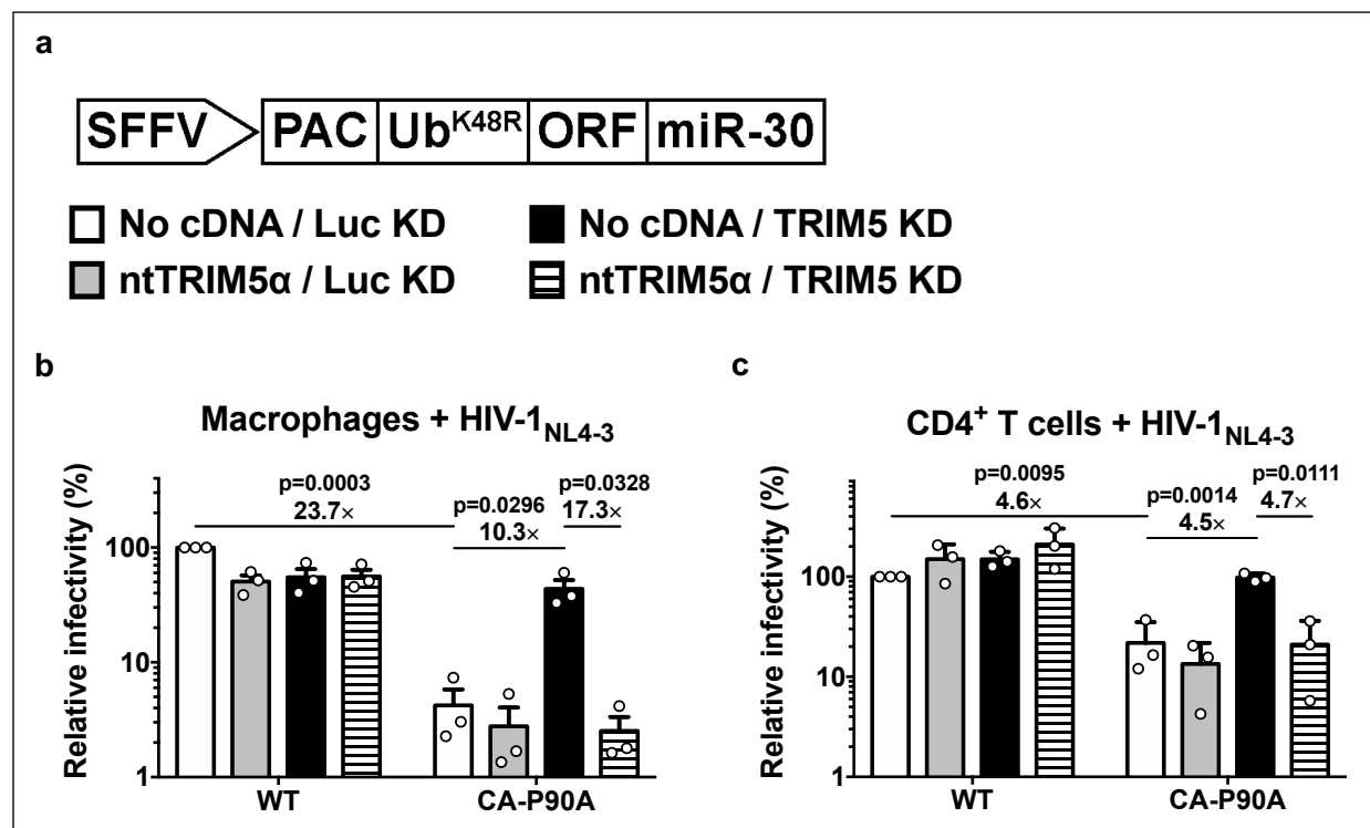
Fig. 2. Human TRIM5 \alpha is sufficient to explain the HIV-1 inhibition that results from disruption of the CA-CypA interaction. a , Schematic representation of the all-in-one shRNA-rescue lentivector, in which the SFFV promoter expresses a tripartite fusion of puromycin N-acetyl transferase (PAC), the K48R mutant of ubiquitin, and an open reading frame for a gene of interest (ORF), as well as a miR-30 based shRNA (miR-30). b and c , All-in-one lentivectors encoding the shRNAs and ORFs indicated in a were used to transduce macrophages ( b ) or CD4 + T cells ( c ). The percentage of GFP-expressing cells was measured by flow cytometry and normalized to the values for No cDNA/Luc KD cells challenged with WT CA; mean \pm SEM, n = 3 donors for each. Significance was determined by two-tailed, paired t-test.
