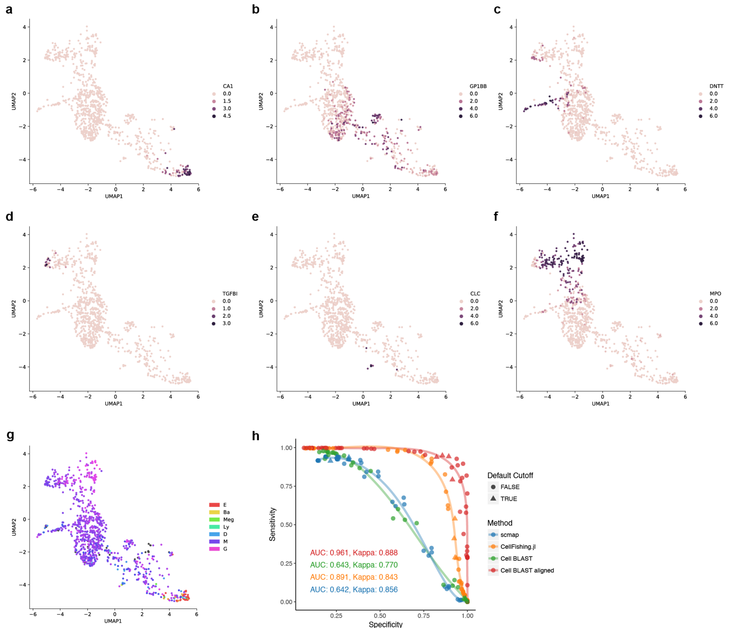
Supplementary Fig. 11 Using “online tuning” in hematopoietic progenitor and Tabula Muris 18 spleen data.
