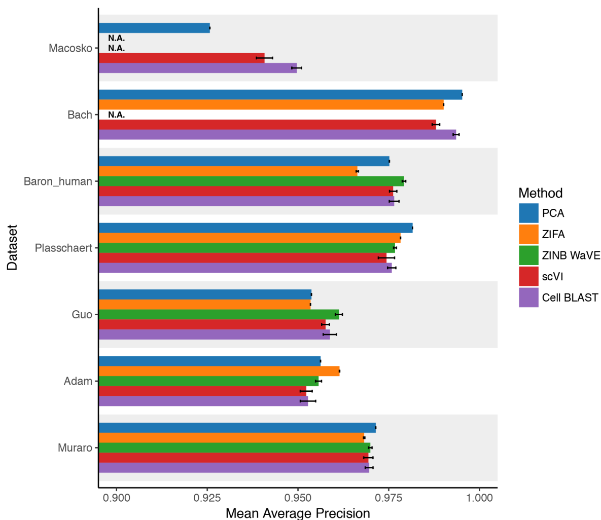
Supplementary Fig. 1 Comparing low-dimensional space cell type resolutions of different dimension reduction methods.
