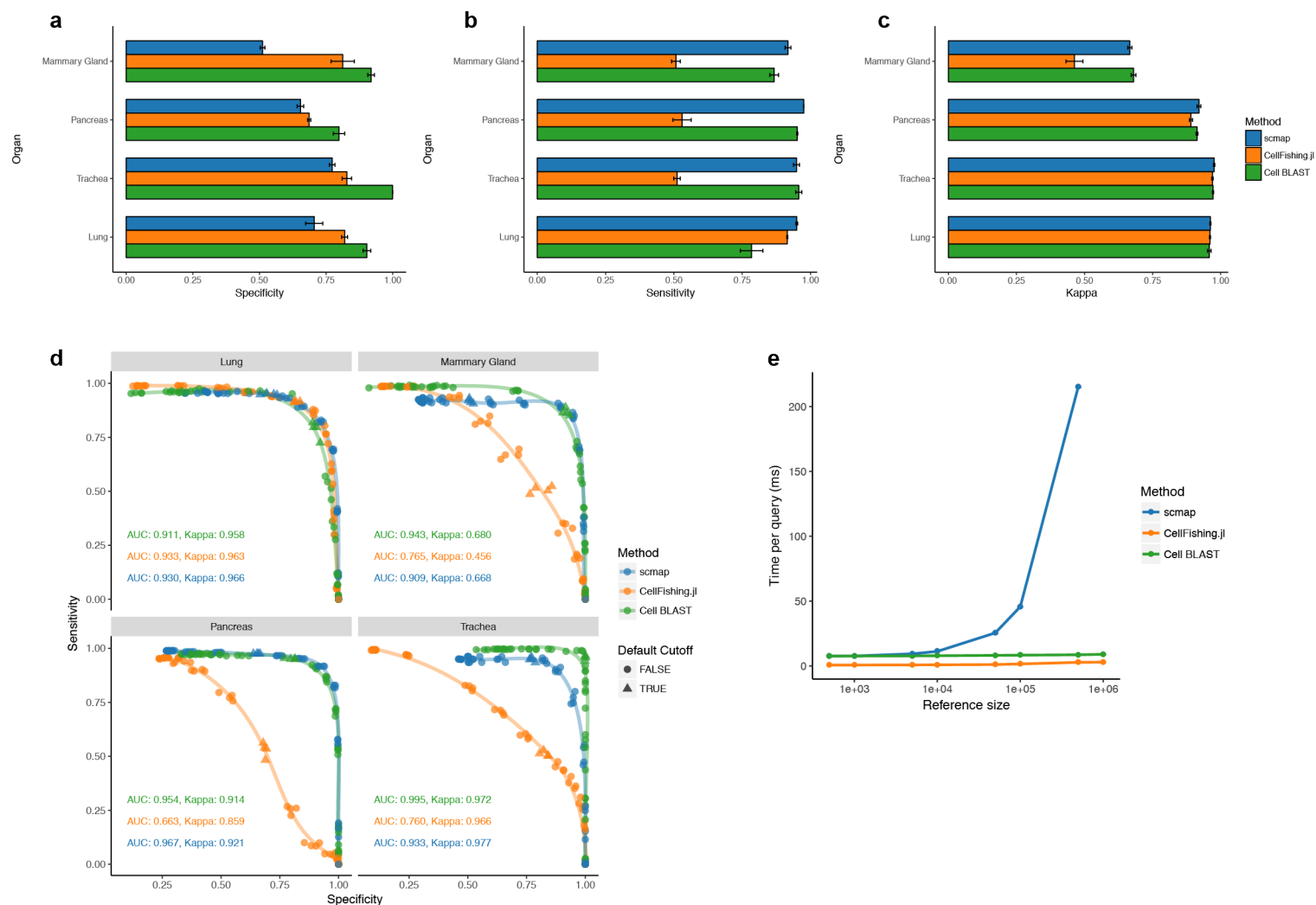
Supplementary Fig. 7 Benchmarking query-based cell typing.
