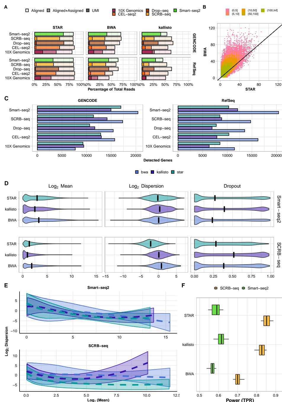
Figure 2. Expression Quantification.
