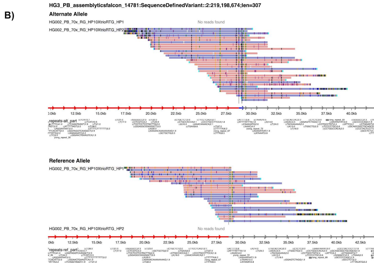
Figure 1. SVCurator web application interface. A) 13 read aligned and dotplot images from svviz2 for several technologies were also visible in addition to the IGV image shown here. B) Svcv2 haplotype separated read aligned image for a 307bp insertion
