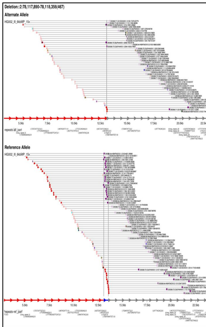
D) svviz2 read aligned image - Illumina Mate Pair (read length = 100 bps; insert size = 6000bp; read depth = 13-14x)
