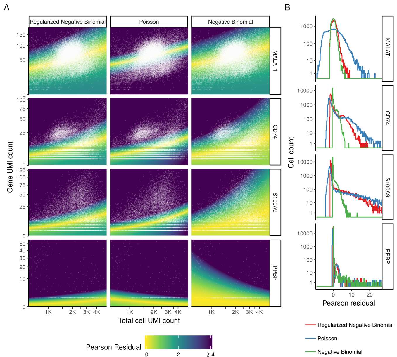
Figure 5: The regularized NB model is an attractive middle ground between two extremes. A) For four genes, we show the relationship between cell sequencing depth and molecular counts. White points show the observed data. Background color represents the Pearson residual magnitude under three error models. For MALAT1 (does not vary across cell types) the Poisson error model does not account for overdispersion, and incorrectly infers significant residual variation (biological heterogeneity). For S100A9 (a CD14+ Monocyte marker) and CD74 (expressed in antigen-presenting cells) the non-regularized NB model overfits the data, and collapses biological heterogeneity. For PPBP (a Megakaryocyte marker) both non-regularized models wrongly fit a negative slope. B) Boxplot of Pearson residuals for models shown in A. X-axis range shown is limited to [-8, 25] for visual clarity.
