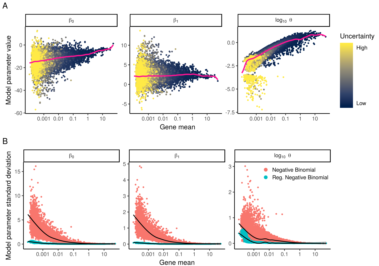
Figure 2: We fit NB regression models for each gene individually, and bootstrapped the process to measure uncertainty in the resulting parameter estimates. A) Model parameters for 16,809 genes for the NB regression model, plotted as a function of average gene abundance. The color of each point indicates a parameter uncertainty score as determined by bootstrapping (Methods). Pink line shows the regularized parameters obtained via kernel regression. B) Standard deviation ( \sigma ) of NB regression model parameters across multiple bootstraps. Red points: \sigma for unconstrained NB model. Blue points: \sigma for regularized NB model, which is substantially reduced in comparison. Black trendline shows an increase in \sigma for low-abundance genes, highlighting the potential for overfitting in the absence of regularization.
