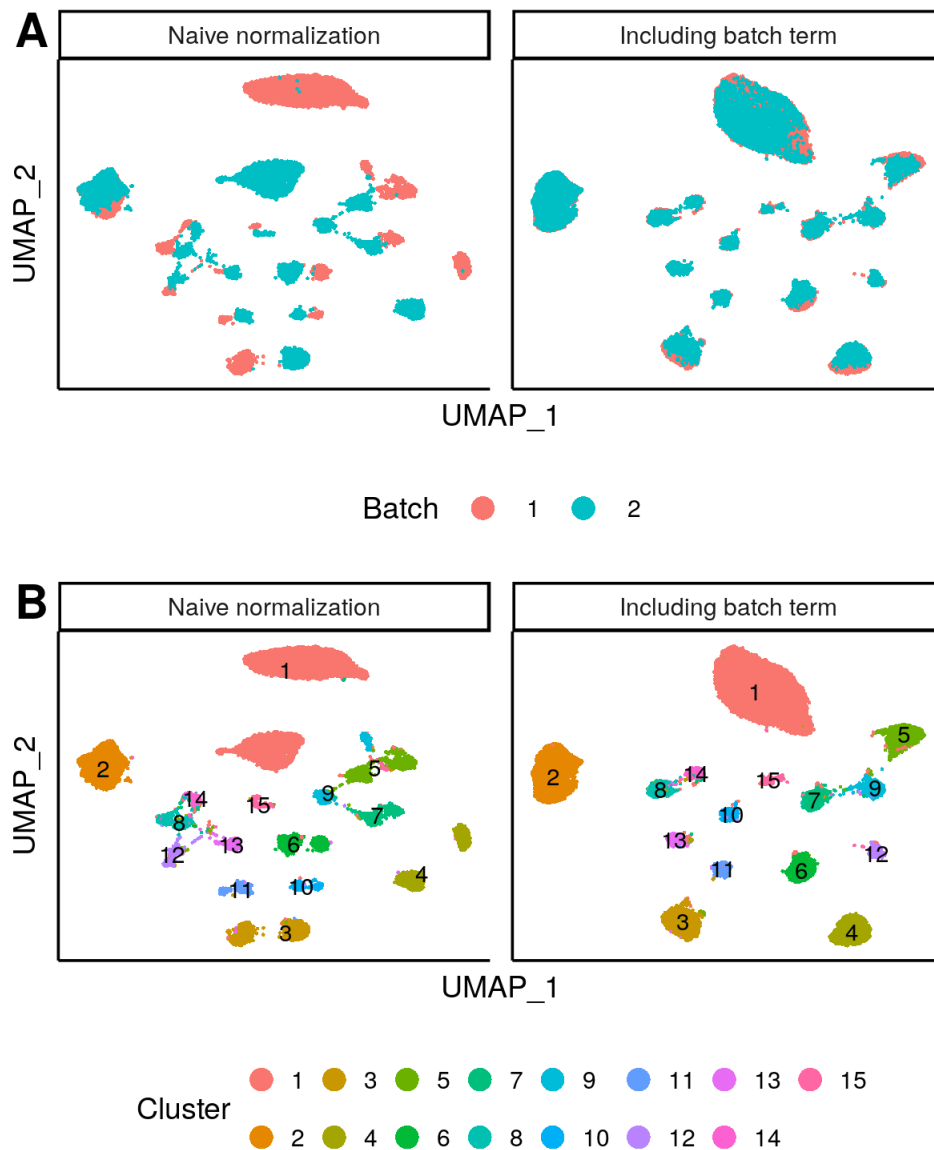
Supp. Figure 3: Batch-correction during normalization. A) UMAP embedding of the bipolar cell dataset before and after including a batch term during normalization. When applying sctransform without the batch indicator variable (i.e. batch-naive normalization), we see clear separation per batch, but when including a batch term in the regression model used for normalization, the batches align. B) Same as above, but colors indicate clusters of the original study. We include this example as a demonstration for how additional nuisance parameters can be included in the GLM framework, but note that when cell-type specific batch effects are present, or there is a shift in the percentage of cell types across experiments, non-linear batch effect correction strategies are needed. Stuart et al. [2018]
