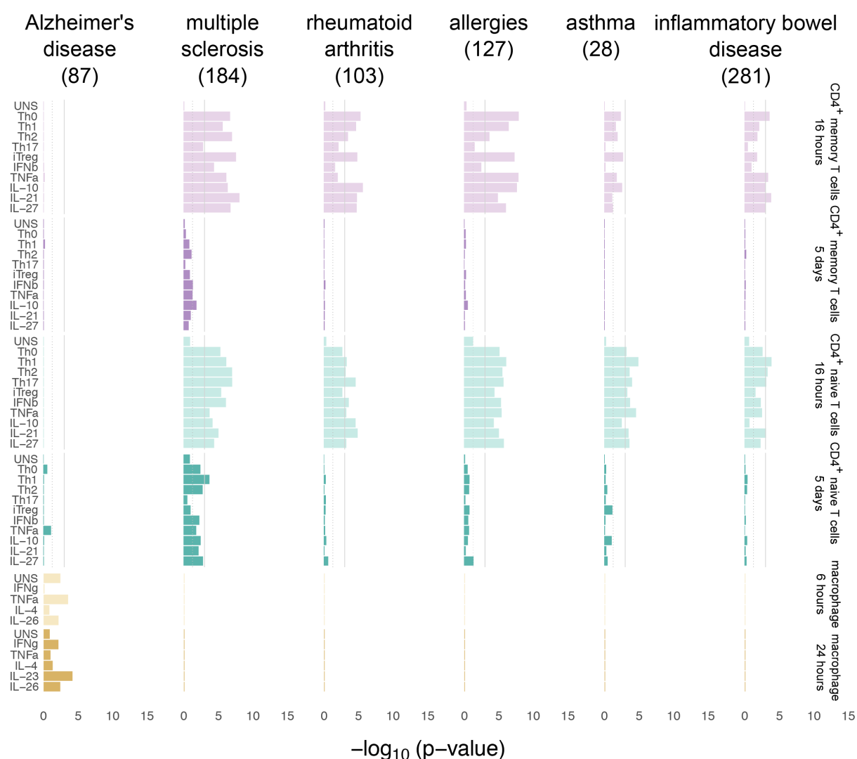
Figure S5. CHEERS SNP enrichment in open chromatin regions in cytokine induced cell states. The numbers in parentheses represent number of overlapping peaks per disease. The dotted gray line represents the nominal p-value threshold of 0.05, while the solid gray line represents the Bonferroni corrected p-value threshold of 0.00091 (corrected for the number of cell states in the study).
