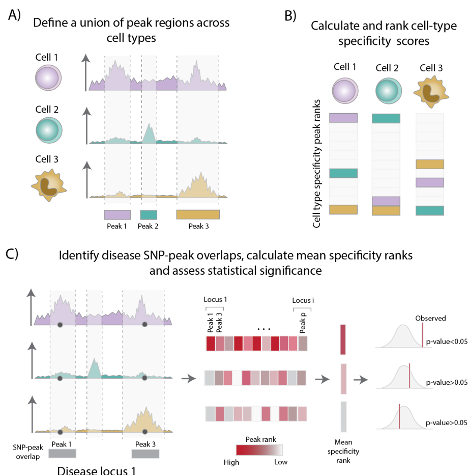
Figure 2. Overview of the CHEERS method. A) We first define a union of peak regions present across cell types and construct a matrix of normalized read counts. B) We then calculate and rank specificity scores. C) To test for disease SNP enrichment, we take all the index variants and identify variants in strong LD ( r^2 > 0.8 ). We then identify peaks that overlap with the associated variants, calculate the mean specificity ranks and assess statistical significance.
