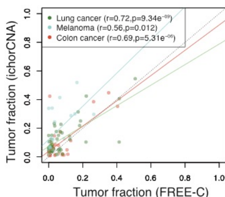
Supplementary Figure 15: Correlation between tumor fraction estimated from ichorCNA and from single-sample FREE-C, using only genomic bins with no overlap of CNVs detected by ichorCNA. Data are plotted as in Figure 4d.
