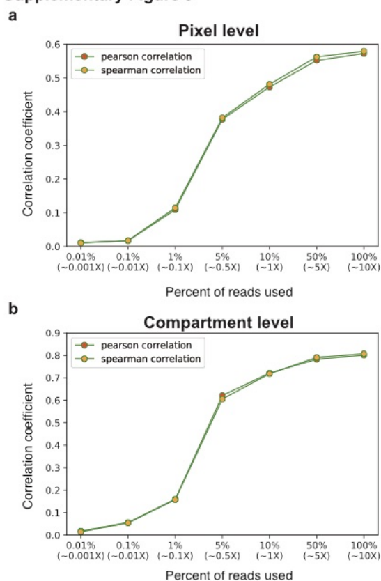
Supplementary Figure 9: Correlation between Hi-C and single-sample FREE-C at different coverages. Pearson and Spearman correlation at pixel level (a) and compartment level (b) between Hi-C (WBC) and single-sample FREE-C (FH1AB8) at different read number after downsampling.
