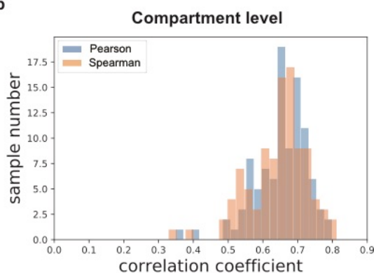
Supplementary Figure 4: The correlation between Hi-C (WBC) and FREE-C at the single sample.
