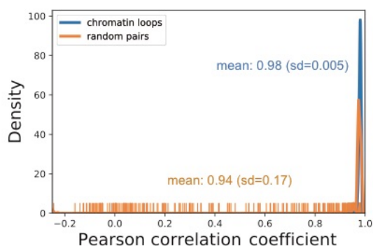
Supplementary Figure 1. Spatial co-fragmentation patterns of cfDNA in multiple human plasma samples. Summary density plot of Pearson correlation coefficient between median fragment length in paired regions identified by HiCCUPS loops called from Arima-HiC in WBC (blue color) and between random pairs of regions with the same distance as the loop (orange color). Additional rug plot on x-axis is plotted to show the long tails in random pairs.
