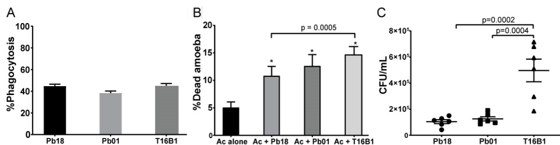
Figure 5. Interaction of Paracoccidioides spp strains with A. castellanii at six hours. Amoebae and three different strains of Paracoccidioides spp (Pb18 – P. brasiliensis , Pb01 – P. lutzii , T16B1 – P. brasiliensis isolated from an armadillo spleen) were co-incubated at a MOI of two at 28 °C. A) Percentage of A. castellanii cells interacting with Paracoccidioides spp. The interaction was assessed by counting at least 100 phagocytes cells per replicate of each sample after Giemsa staining of the samples. The bars represent 95% confidence intervals. B) Viability of A. castellanii upon interaction with Paracoccidioides spp. The viability was assessed by counting at least 100 cells per replicate of each sample after staining with trypan blue. The bars represent means plus 95% confidence intervals. C) Survival of fungal cells from different strains of Paracoccidioides spp following interaction with amoebae. The error bars represent standard error of the mean. Figures depict the combined results of at least three independent experiments. *All the strains showed a significant difference in the % of dead amoebae at six hours relative to the control amoebae growing alone.
