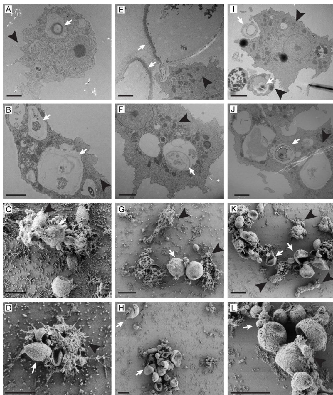
Figure 3– TEM and SEM analysis of the interaction of P. brasiliensis Pb18 cells and different soil amoebae. The isolates were co-incubated with Pb18 at a MOI of five at 25 °C for 24 h in PAS and fixed for microscopy. A-B) TEM of the interaction of P. brasiliensis with A. spelaea . Scale bars = 500 nm. C-D) SEM of the interaction of P. brasiliensis with A. spelaea . Scale bars = 10 µm. E-F) TEM of the interaction of P. brasiliensis with Acanthamoeba spp. Scale bars = 2 µm. G-H) SEM of the Interaction of P. brasiliensis with Acanthamoeba spp. Scale bars = 10 µm. I-J) TEM of the interaction of P. brasiliensis with V. vermiformis . Scale bars = 2 µm. K-L) SEM of the interaction of P. brasiliensis with V. vermiformis . Scale bars = 10 µm. White arrows indicate fungal cells, or their remains and black arrow heads indicate amoeba cells.
