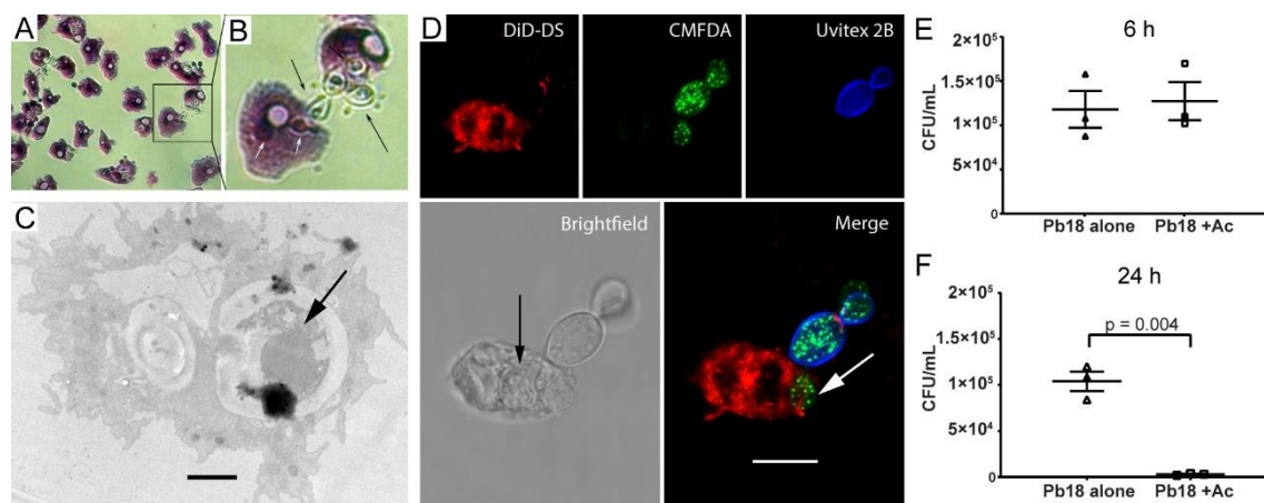
Figure 4- P. brasiliensis Pb18 interaction with an axenic Acanthamoeba castellanii strain. A) P. brasiliensis and A. castellanii were co-incubated at a MOI of one for one hour at 28 °C, and then stained with Giemsa and observed by light microscopy. B) Enlargement of the area depicted in the square region of panel A. C) TEM of the interaction of A. castellanii and Pb18 cells. Incubation was at a MOI of one for six hours at 28 °C and then fixed. The black arrow indicates an internalized P. brasiliensis (Scale bar = 2 µm). D) Confocal microscopy. A. castellanii was dyed with DiD-DS (red), while P. brasiliensis cells were labeled first with CMFDA (green), and after the interaction with Uvitex 2B (blue). The arrows show fungal cells inside an amoeba. (Scale bar = 10 µm). E and F) Survival of P. brasiliensis after interaction with A. castellanii interaction. Incubation was at a MOI of two at 28 °C for six ( E ) or 24 hours ( F ), using the fungus alone as a control. After the interaction amoeba cells were lysed and fungal cells were plated for CFU counting. The figure depicts the results of three independent experiments. The error bars represent standard error of the mean.
