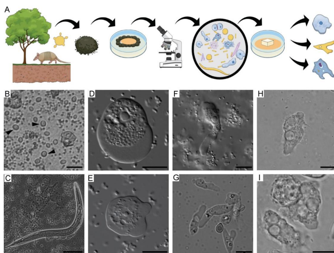
Figure 1– Soil organisms sharing the putative habitat of P. brasiliensis . A) Schematic representation of the soil amoeba isolation methodology. Soil samples from armadillo burrows positive for P. brasiliensis DNA were collected and used for the isolation of soil amoebae. The samples were plated in non-nutrient agar plates containing a bacterial lawn as food source and observed in an inverted microscope B) Bright field microscopy of trophozoites of ciliates (black arrow heads) present in a soil sample. Scale bar = 20 \mu m, C) Bright field microscopy of a nematode present in the soil sample. Scale bar = 50 \mu m, D) and E) DIC microscopy of trophozoites of A. spelaea . Scale bar = 10 \mu m. F) and G) DIC microscopy of trophozoites of V. vermiformis . Scale bar = 10 \mu m. H) and I) DIC microscopy of trophozoites of Acanthamoeba spp. Scale bar =10 \mu m.
