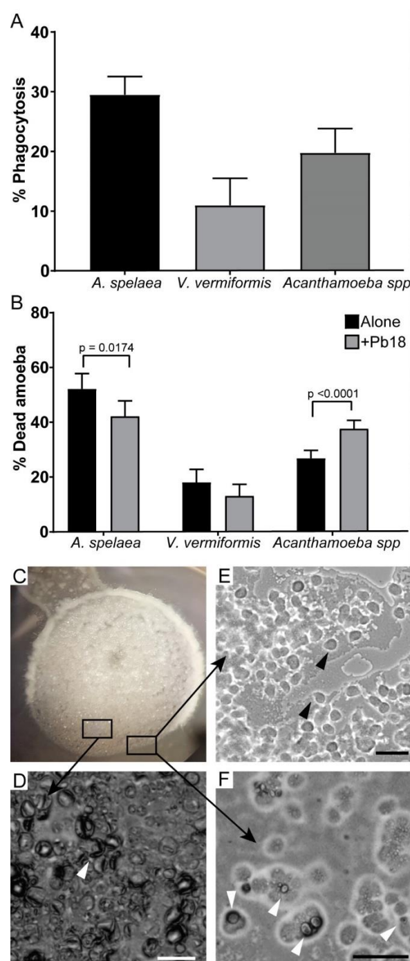
Figure 2– Interaction of P. brasiliensis Pb18 with amoebae isolated from soil of armadillo burrows positive for P. brasiliensis . The amoeba isolates were co-incubated with Pb18 previously dyed with pHrodo™ or FITC at a MOI of two at 25 °C for 24 h in liquid medium. A) Percentage of amoeba cells interacting with P. brasiliensis Pb18. After the interaction Pb18 cells were dyed using Uvitex 2B. B) Viability of the different amoeba isolates after 24 h of interaction with Pb18. A and D depicts the results of at least three independent experiments. At least 100 cells per replicate of each sample were counted for each assay. The bars represent 95% confidence intervals. C-F a suspension of A. spelaea cells was dropped next to a colony of P. brasiliensis cells in non-nutrient agar. The cells were co-incubated at 25 °C and examined daily in an inverted microscope. C) Macroscopic view of the fungal colony in a 35 mm plate. D) Microscopic view of the fungal cell lawn after seven days of interaction. E) Microscopic view of amoeba trophozoites growing in the periphery of the fungal lawn. F) Microscopic view of amoeba trophozoites interacting with a fungal cell. Scale bars = 50 \mu m. Black arrow heads indicate trophozoites. White arrow heads indicate fungal cells.
