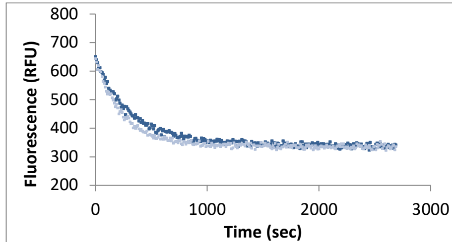
Figure 5: Effects of tetraUb on Nucleotide Exchange
