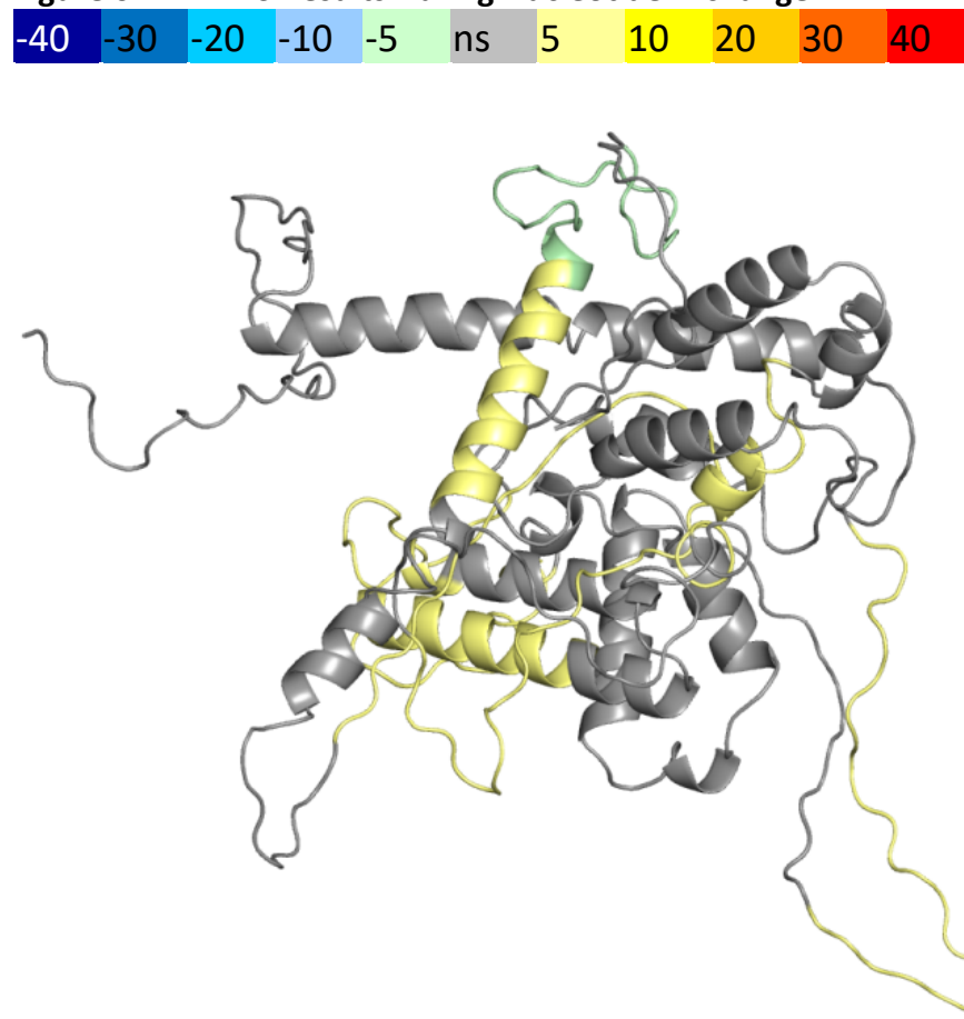
Figure 6: HDX-MS Results During Nucleotide Exchange
