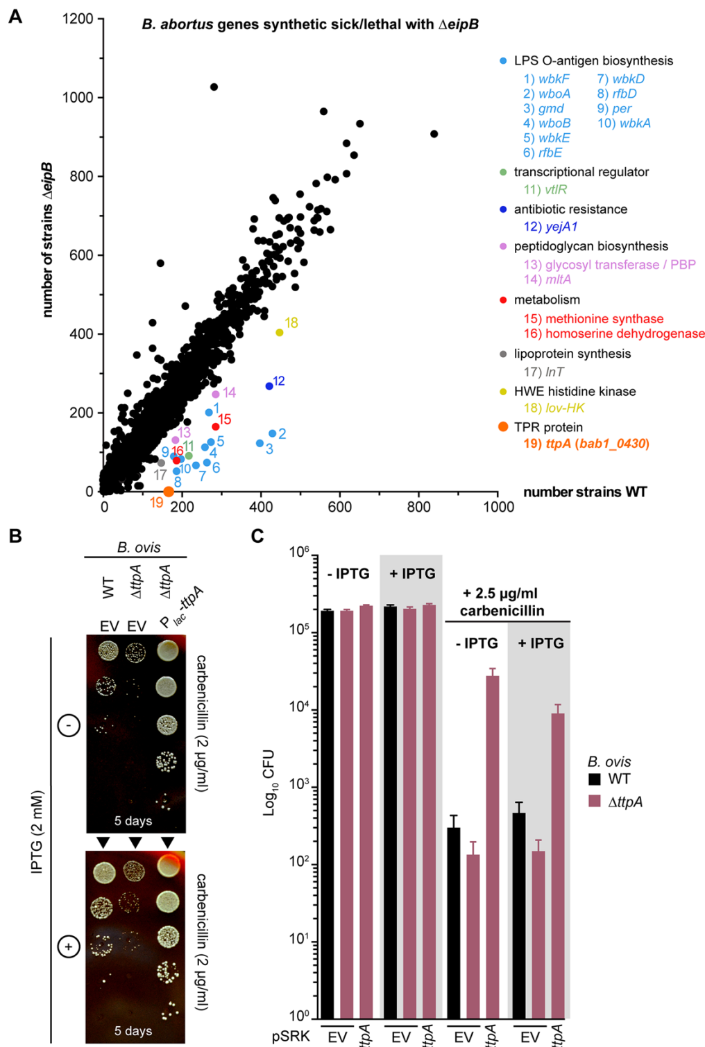
Figure 8: B. abortus eipB deletion is synthetically lethal with Tn-Himar disruption of bab1_0430 , which encodes a tetratricopeptide repeat (TPR) protein. A) Identification of B. abortus genes that are synthetically lethal or sick with eipB deletion. Tn-Himar insertion strains per gene (black dots) obtained in a B. abortus \Delta eipB background are plotted as a function of strains per gene in a wild-type background. bab1_0430 , for which we observed significantly fewer insertions in \Delta eipB than
