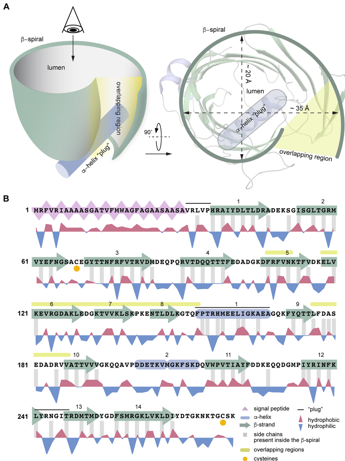
Figure 6: Simplified representation of EipB structure. A) EipB adopts a cup-like structure, fourteen \beta -strands (in green) form an overlapping \beta -spiral ( \beta 5- \beta 6- \beta 7- \beta 8 overlap with \beta 9- \beta 10 connecting loop, highlighted in yellow in panel A and B). \alpha 1 (in violet) and the loop connecting \beta 12 and \beta 13 form the bottom of this "cup". B) Amino acid sequence of EipB. The sequence corresponding to
