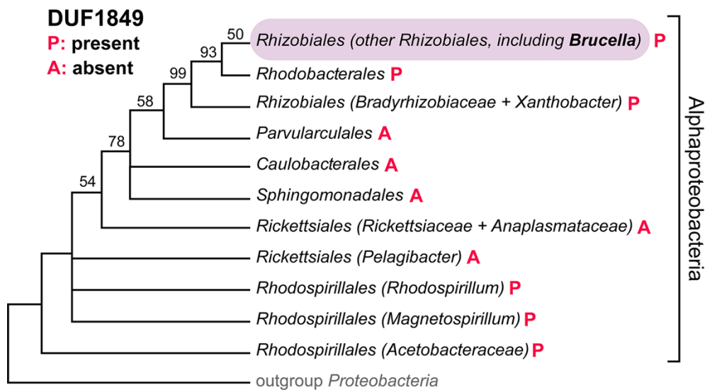
Figure 1: The DUF1849 sequence family is restricted to Alphaproteobacteria. Bayesian phylogenetic tree showing the distribution of DUF1849 genes in different orders within the class Alphaproteobacteria (P: present, A: absent). Bayesian support values are shown when <100%; nodes were collapsed when support was <50%; adapted from Williams and colleagues (50). In Brucella abortus (order Rhizobiales), DUF1849 is encoded by gene locus bab1_1186 (i.e. eipB ).
