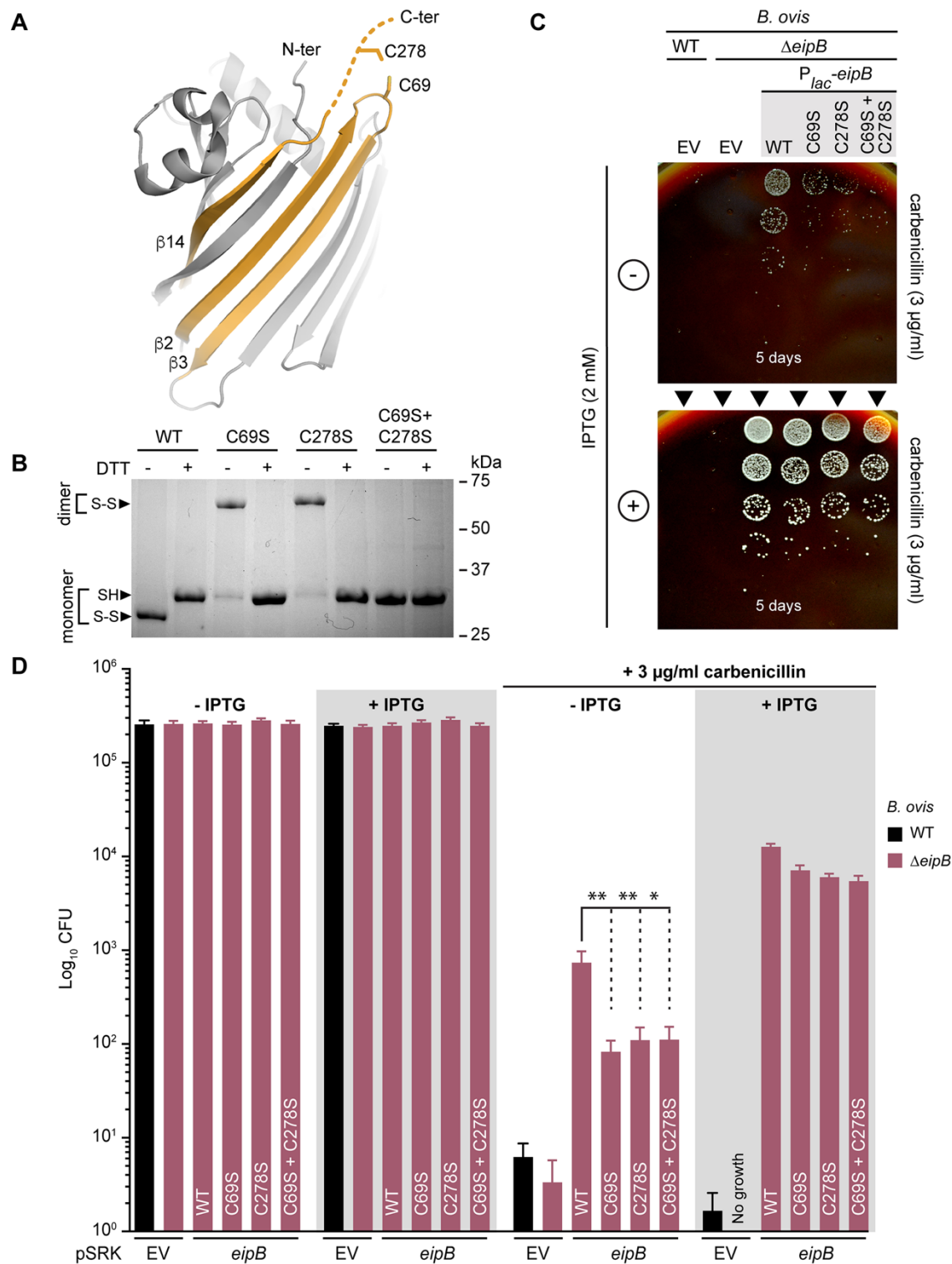
Figure 7: EipB has an internal disulfide bond. A) Cysteines C69 and C278 are spatially proximal in the EipB structure and form a disulfide bond. C278 is present at the EipB C-terminus that follows \beta 14, and C69 is present in a loop connecting \beta 2 and \beta 3. B) His-tagged wild-type EipB and EipB cysteine mutant proteins (C69S, C278S, and C69S+C278S) were purified and mixed with a protein loading buffer plus or minus 1 mM DTT. Protein samples were resolved by 12% SDS-PAGE. This
