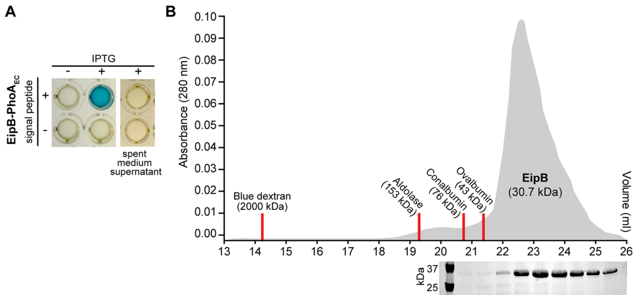
Figure 4: EipB is monomeric in solution and is secreted to the Brucella periplasm. A) Alkaline phosphatase assay. Overnight cultures of B. ovis expressing EipB with (+) or without (-) its signal peptide and fused to E. coli PhoA, were grown in presence (+) or absence (-) of 1 mM IPTG inducer. In a 96-well plate, these cultures were mixed with BCIP (200 \mu M final concentration) and developed for 2 hours at 37°C / 5% CO 2 . Only the strain expressing EipB-PhoA Ec with a signal peptide turned blue, providing evidence that the protein is located in the periplasm. As a control, spent medium supernatants were mixed with BCIP to test whether EipB-PhoA Ec is secreted into the medium. After 2 hours incubation, no color change was observed, indicating that EipB-PhoA Ec is not exported outside the cell. These experiments were performed at least three times with independent clones. A representative image is shown. B) Size exclusion chromatography elution profile of purified EipB (in grey). Elution fractions were loaded on a SDS-PAGE, and a single band migrating at ~30 kDa was visible. Elution peaks of the molecular weight standards (blue dextran: 2000 kDa, aldolase: 157 kDa, conalbumin: 76 kDa, ovalbumin: 43 kDa) are shown as red line. This experiment was performed twice and yielded similar elution profiles.
