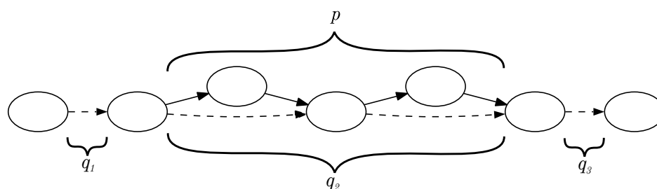
Figure 6: An example of computing the score of a walk p (solid) relative to an ancestral path p_a = q_1 q_2 q_3 (dashed). The path p forms a chain with the subpath q_2 of p , while subpaths q_1 and q_3 form “hanging ends”. We count the length of p and subtract lengths of the hanging ends. Thus, the score f(p_a, p) = 4 - 1 - 1 = 2 .
