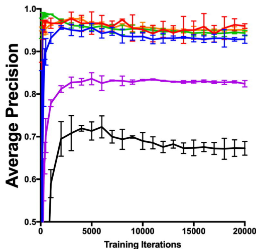
B Faster-RCNN trained on individual datasets with additional vertically flipped data augmentation
