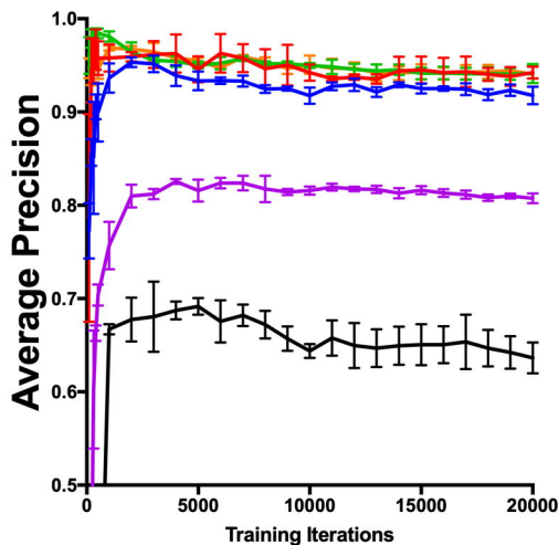
A Faster-RCNN trained on individual datasets with no additional data augmentation
