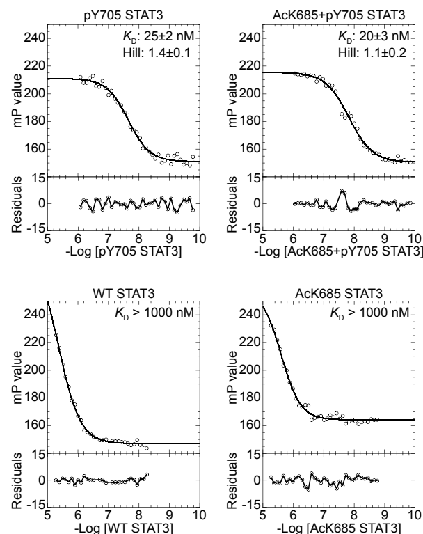
Figure 1: Affinity of STAT3 variants to the \alpha 2M promoter, measured by fluorescence anisotropy. Increasing concentrations of the indicated STAT3 proteins were incubated with 2 nM of 3'-fluorescein-labeled probe, and data were fitted to Equation 1. Average K_D and Hill slope values are displayed ( n=3 , \pm SD). The affinity of non-phosphorylated STAT3 variants was below the detection limit. mP: millipolarization units.
