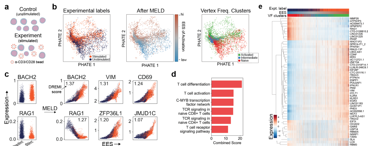
Figure 3: MELD recovers signature of TCR activation. (a) Jurkat T-cells were stimulated with \alpha -CD3/CD28 coated beads for 10 days before collection for scRNA-seq. (b) Examining a PHATE plot, there is a large degree of overlap in cell state between experimental conditions. However, after MELD it is clear which cells states are prototypical of each experimental condition. (c) Relationship between gene expression and TCR activation state is revealed when cells are ordered by the EES instead of grouped by experimental condition. (d) Signature genes identified by top 1% of kNN-DREMI scores are enriched for annotations related to TCR activation. (e) Z-scored expression of select signature genes ordered by the EES reveals patterns of up- and downregulation. Notice a subset of genes exhibit non-monotonic expression patterns, such as USP14 and NSRP1. Identifying such trends would be impossible without MELD.
