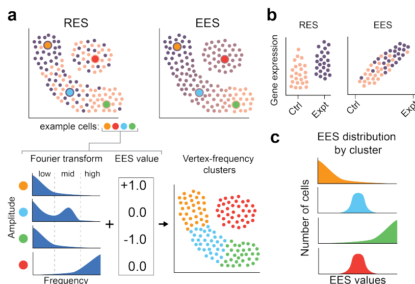
Figure 2: Clustering and Experimental Analysis with MELD (a) The Windowed Graph Fourier Transform and EES values at four example points shows distinct patterns between a transitional (blue) and unaffected (red) cell. This information is used for Vertex Frequency Clustering. (b) Ordering cells by the EES reveals gene expression changes of the experimental condition. (c) Examining the distribution of EES scores in vertex-frequency clusters identifies cell populations most affected by a perturbation.
