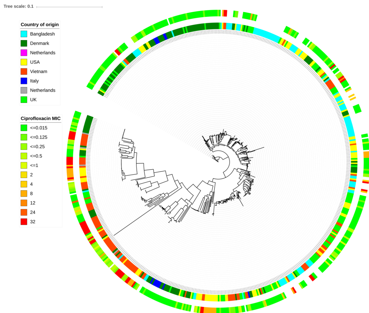
Figure 3: Maximum likelihood tree based on the alignment of concatenated core genes of 572 E. coli genomes (5 genomes failed quality control or assembly). Country of origin (inner circle) and ciprofloxacin minimum inhibitory concentration (outer circle) are indicated for each isolate. Zone diameters values for antibiotic susceptibility were not included in this analysis (isolates from Bangladesh).
