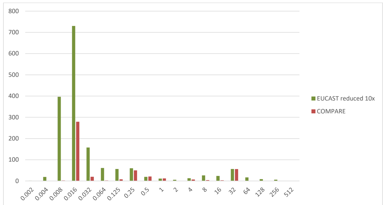
Figure 2: Distribution of the E. coli ciprofloxacin MICs and comparison with ECOFFs ( https://mic.eucast.org/Eucast2/ ).
