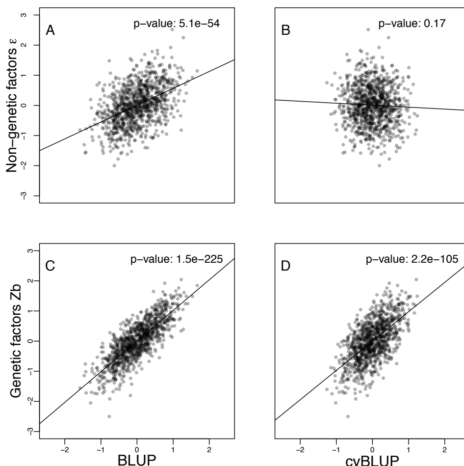
Figure 1. Correlations of genetic predictions, BLUP and cvBLUP, with true genetic factors Zb and independent environmental factors \epsilon in a simulation of a continuous phenotype with h^2 \approx 50\% , 1000 subjects, and 1000 independent SNPs having random effect sizes. BLUPs are correlated with \epsilon while cvBLUPs are not. Lines and p-values are from linear regression fits. R^2 values: A:0.21, B:0.0019, C:0.64, D:0.38.
