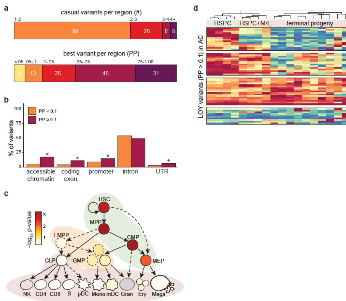
Figure 3 | Results from fine-mapping analyses. Panel a shows the posterior expected number of causal variants ( top ) as well as the best fine-mapped variant ( bottom ) in each region. Genomic enrichments for variants stratified by posterior probability are shown in panel b . Fine-mapped variants were enriched for accessible chromatin in hematopoiesis, as well as in exons, promoters, and UTRs of protein coding genes, but not for introns. Panel c shows g-chromVAR cell-type enrichments across the hematopoietic tree for LOY. HSCs, MPPs, and CMPs meet Bonferroni threshold ( \alpha = 0.05 / 18 ). Developmental patterns of accessible chromatin for variants with posterior probability > 10% are shown in panel d , revealing that 14 variants are fully restricted to acting within HSPCs, 14 variants can also have regulatory effects in myeloid and lymphocyte progenitors, and 17 variants are capable of acting across the majority of hematopoiesis. K-means clustering ( k = 4 determined by the gap statistic) was used to identify patterns of accessibility, and cell types were hierarchically clustered. HSC, hematopoietic stem cell; MPP, multi-potent progenitor; CMP, common myeloid progenitor; HSPC, hematopoietic stem and progenitor cell; M/L, myeloid and lymphoid; PP, posterior probability; AC, accessible chromatin; UTR, untranslated region; PChIC, promoter capture Hi-C; eQTL, expression quantitative trait locus; corr, ATAC/chromatin-RNA correlations
