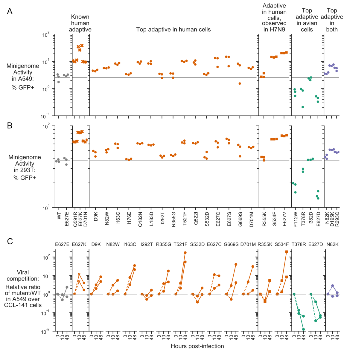
Figure 4. Validation of top experimentally adaptive mutations.
