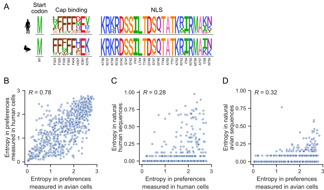
Figure 2. Functional constraints on PB2.
