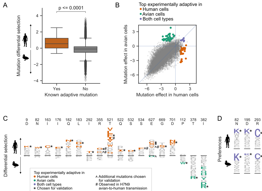
Figure 3. Deep mutational scanning identifies known and novel host-adaptive mutations.
