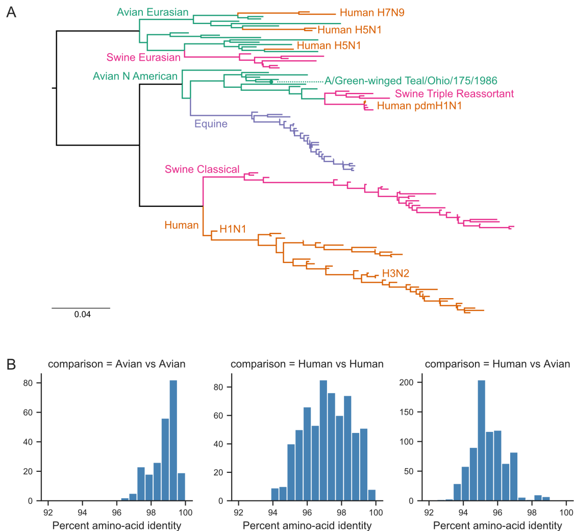
Figure S1. Related to Figure 1. Phylogenetic relationship of PB2 sequence of chosen avian influenza strain to other influenza strains
