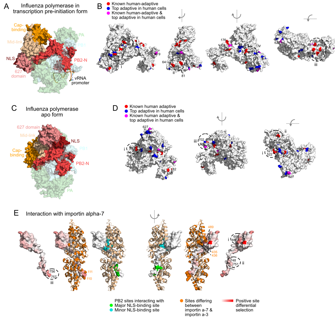
Figure 5. Locations of top human-adaptive mutations on the structure of the influenza polymerase.
