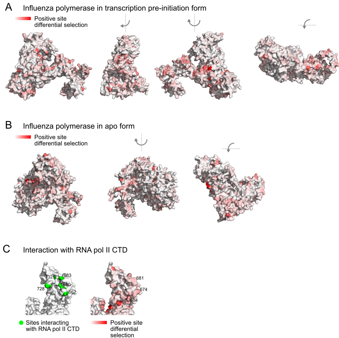
Figure S5. Related to Figure 5. Locations of identified human adaptive mutations on influenza polymerase.
