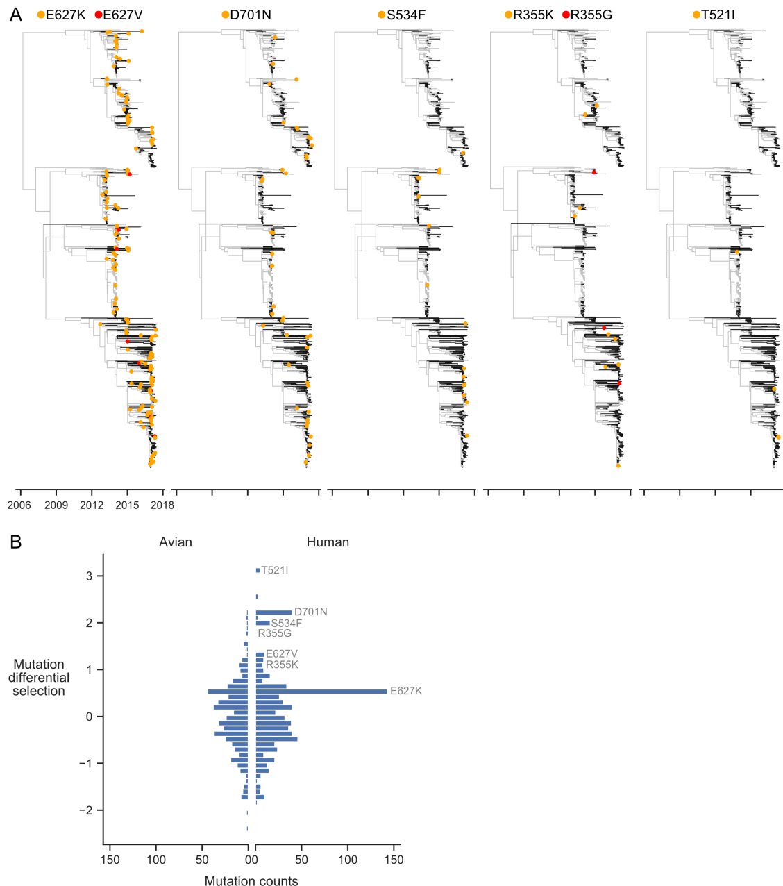
Figure 6. Experimentally identified human-adaptive mutations are enriched in avian-human transmission of H7N9 influenza.
