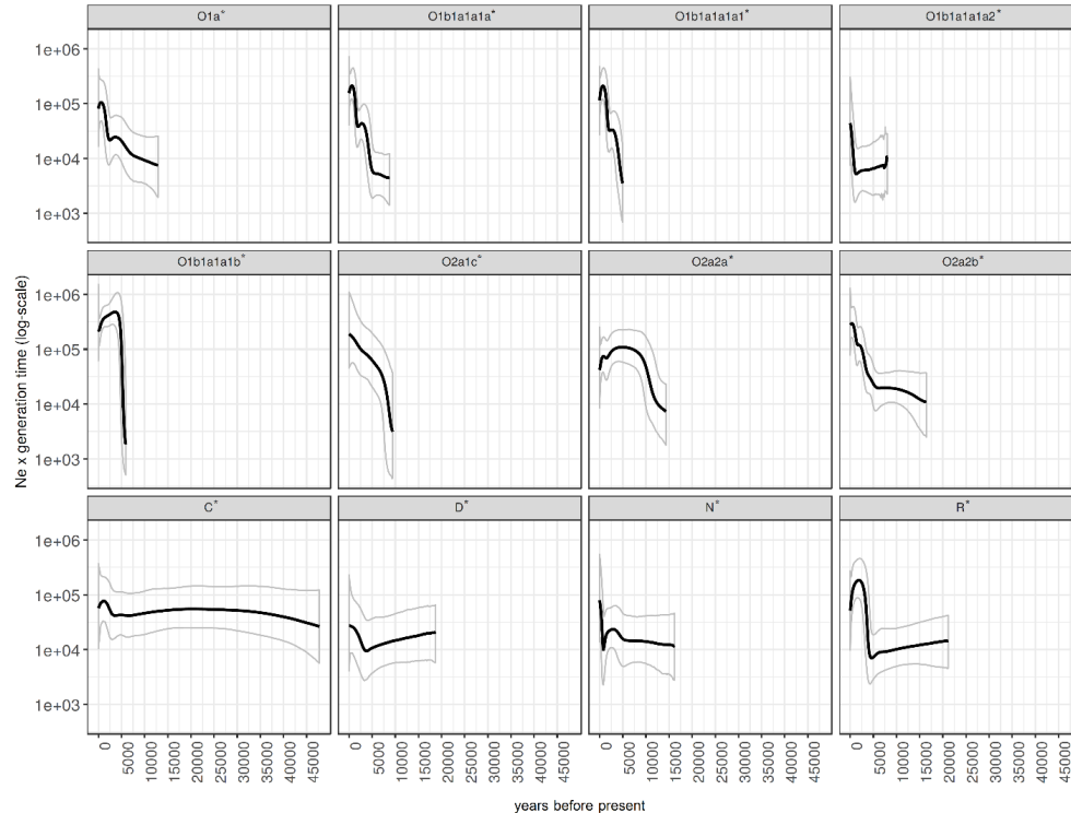
Figure 8 The BSP plots for each major haplogroup. Solid lines are the median estimated paternal effective population size (y-axis) through time from the present in years (x-axis). The 95% highest posterior density limits are indicated by dotted lines.
