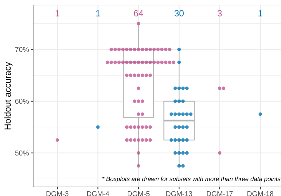
Figure 4: TPOT-DS's holdout accuracy in RNA-Seq expression data with selected subset. Number of pipeline inclusions of each subset in 100 replications is displayed above the boxplots. Subsets DGM-5 and DGM-13 are the most frequent to be included in the final pipeline. Pipelines that include DGM-5, on average, produce higher MDD prediction accuracies in the holdout set.
