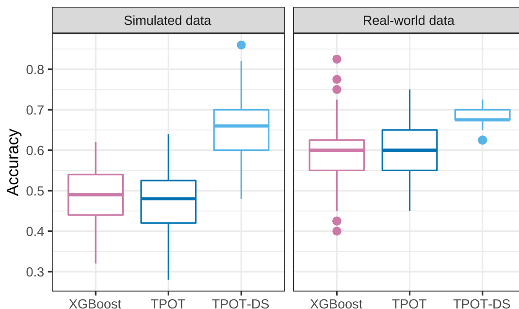
Figure 2: Performance comparison of three models: tuned XGBoost, optimal pipeline from standard TPOT and optimal pipeline from TPOT-DS.
