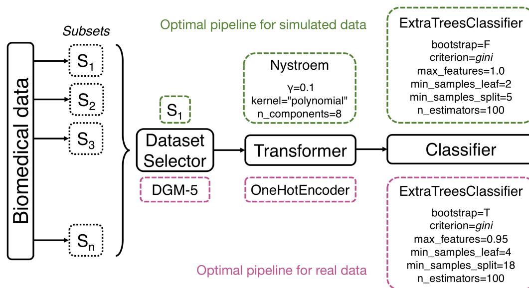
Figure 1: TPOT-DS's workflow and example pipelines. Final pipelines with optimized parameters are shown for simulated data (top) and real-world gene expression data (bottom).
