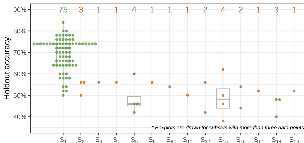
Figure 3: TPOT-DS's holdout accuracy in simulated data with selected subset. Number of pipeline inclusions of each subset in 100 replications is displayed above the boxplots. Subset
