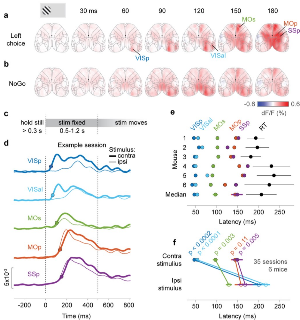
Figure 2 | Sequential activation of cortical areas. a. Average cortical fluorescence (dF/F) over all sessions of one mouse (mouse 1). Columns show successive times relative to stimulus onset, for trials with a stimulus on the left screen only and the mouse made a Left choice. Gray lines: contours of cortical areas defined from the Allen Common Coordinate Framework (CCF; image cropped to this region). Black dot: bregma. b. Same as in (a) but for NoGo trials. Average stimulus contrast was matched between NoGo and Left trials in (a). c. Task timeline during widefield calcium imaging. To distinguish activity associated with initial wheel movement from activity driven by visual motion, we introduced an open-loop period 0.5-1.2 s after grating onset, when wheel movements did not move the grating. Trials were excluded post-hoc if choices were made after this period. d. Stimulus-locked calcium fluorescence at 5 ROIs for one example session from mouse 1. Thick lines are the average response to contralateral stimuli over all correct trials. Thin lines are the same but for trials with only ipsilateral stimuli. Response latency, marked with a dot, is defined as the time for the mean fluorescence across trials to reach 30% of the peak. e. Summary of fluorescence response latencies to the contralateral stimulus for 6 mice (see Methods for genotype information). Rows show data from individual mice, with dots showing each ROI's response latency for trials pooled across sessions. Bottom row: response latencies and reaction time averaged across mice (dots and lines: median \pm m.a.d.). f. Response latencies to contralateral and ipsilateral stimuli for each region, averaged across mice (closed and open circles). Significance was determined by a two-tailed paired t-test, t(5) = -10.38, -12.00, -5.46, -1.97, -4.72 .
